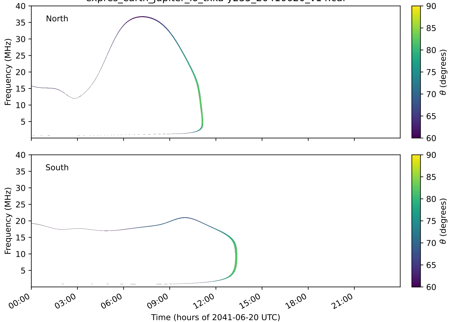
expres_earth_jupiter_io_txka-y235_20410620_v14.cdf
