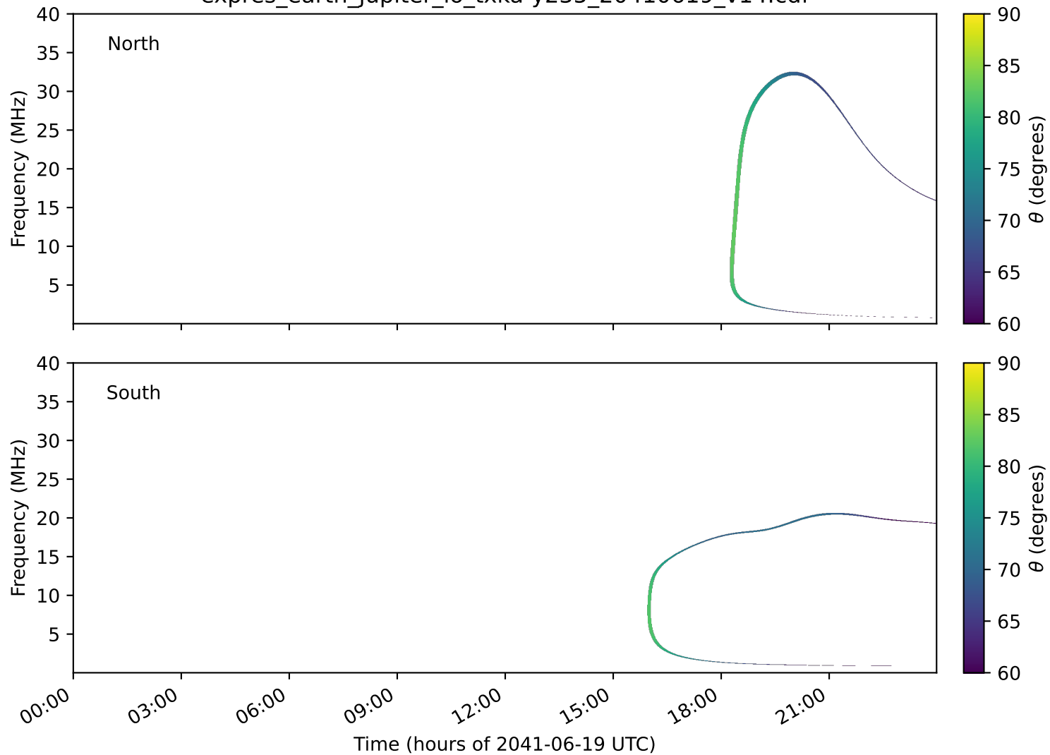
expres_earth_jupiter_io_txka-y235_20410619_v14.cdf
