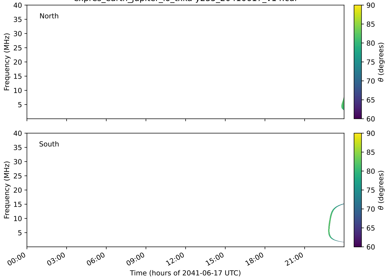
expres_earth_jupiter_io_txka-y235_20410617_v14.cdf
