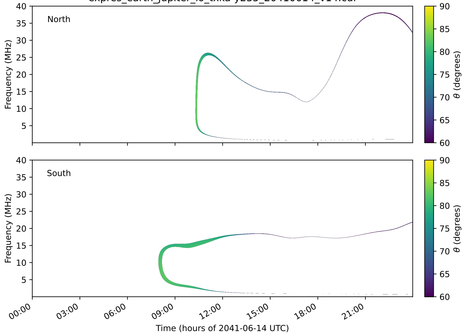
expres_earth_jupiter_io_txka-y235_20410614_v14.cdf
