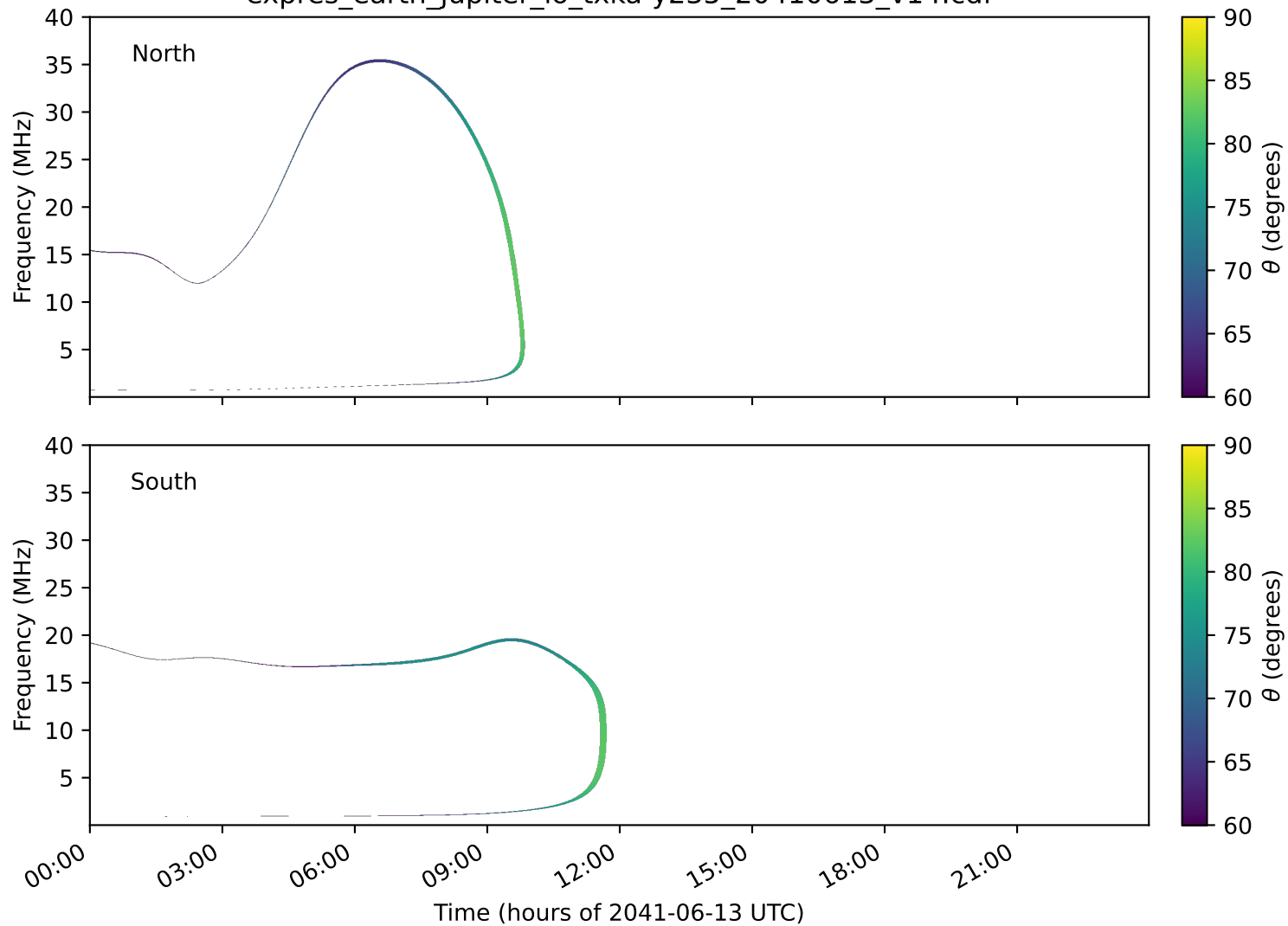
expres_earth_jupiter_io_txka-y235_20410613_v14.cdf
