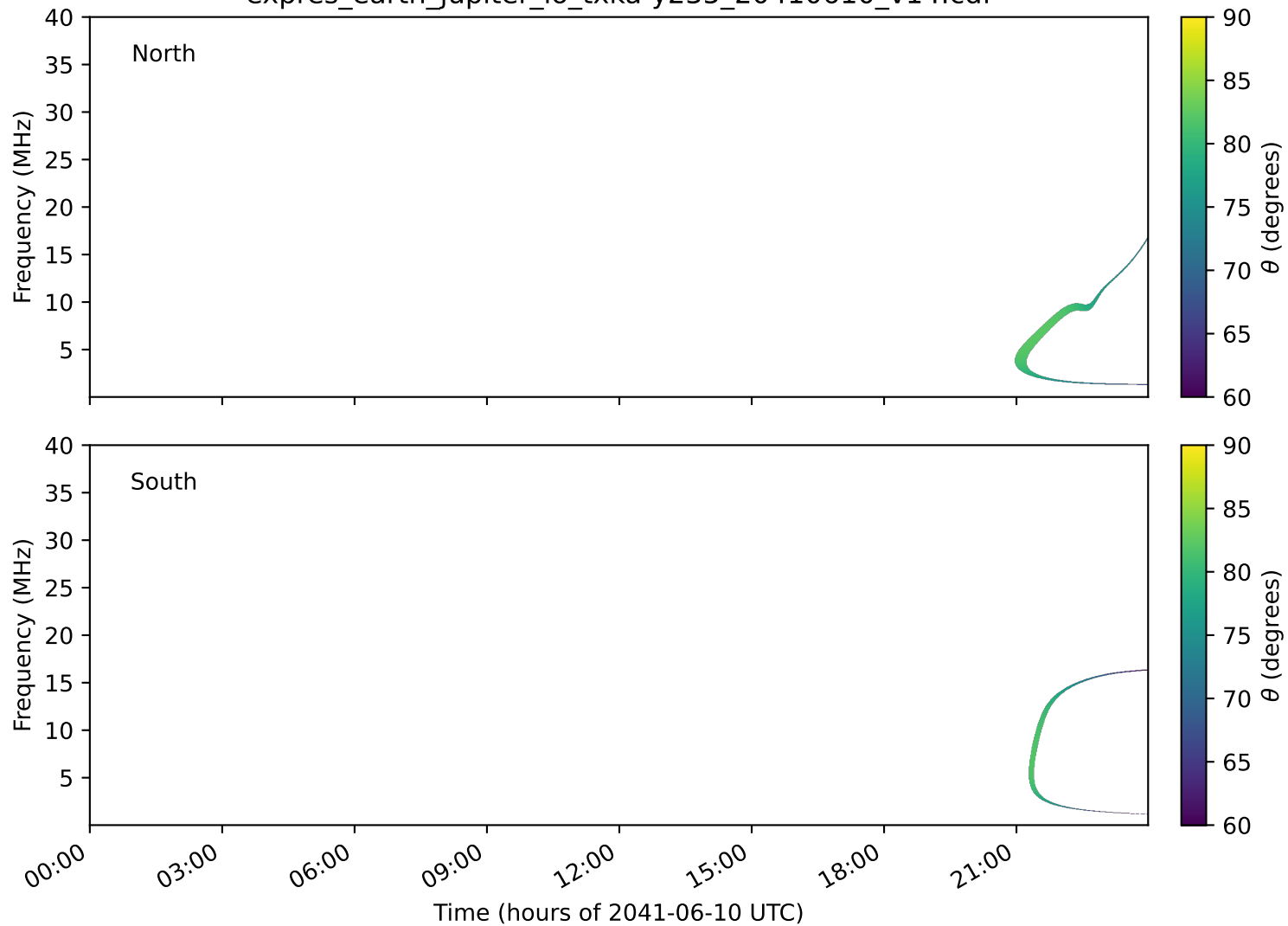
expres_earth_jupiter_io_txka-y235_20410610_v14.cdf
