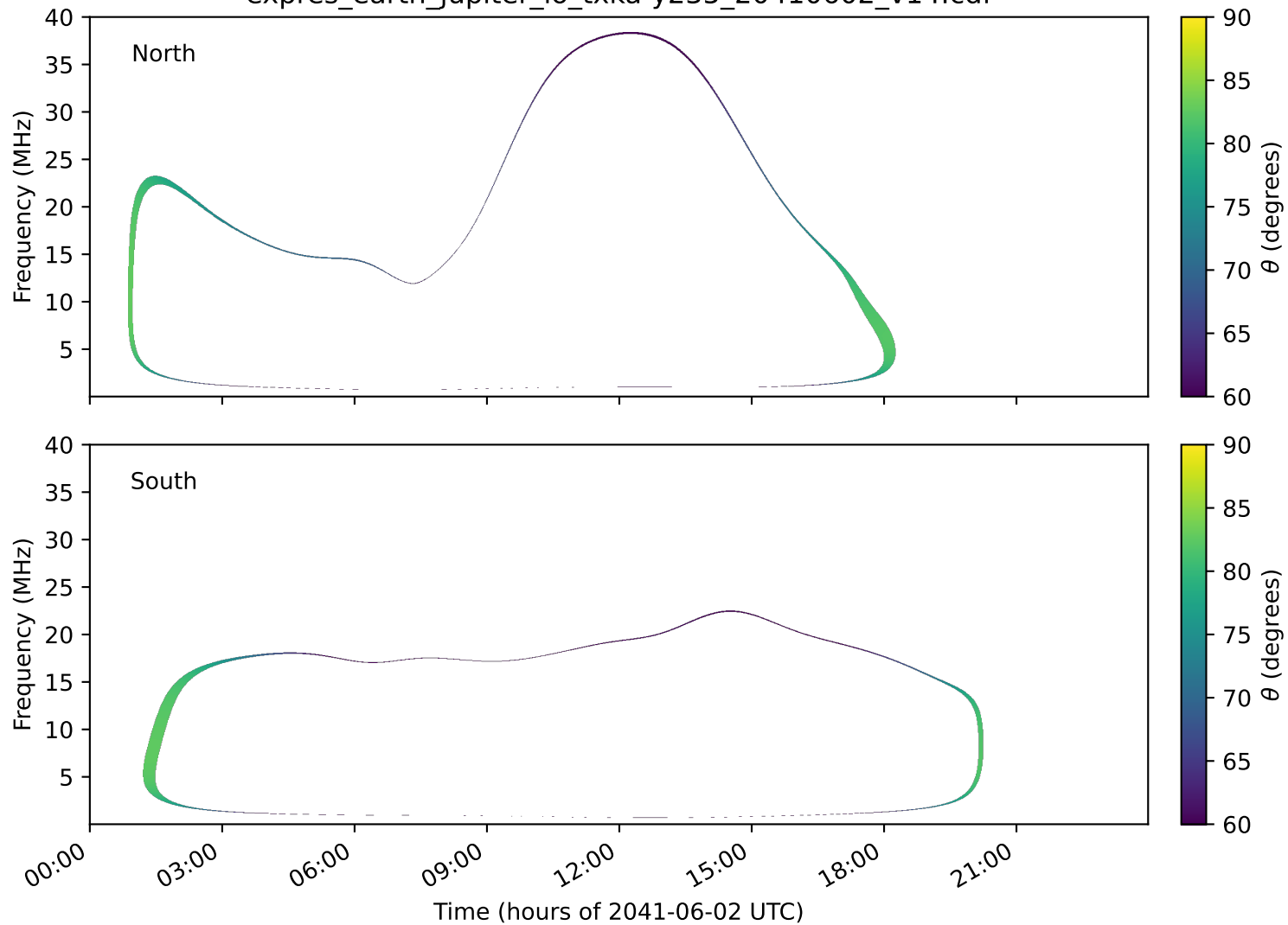
expres_earth_jupiter_io_txka-y235_20410602_v14.cdf
