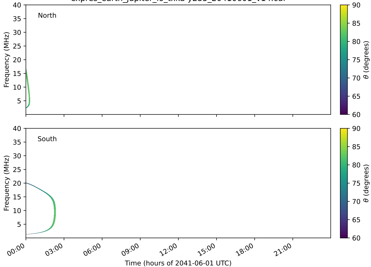
expres_earth_jupiter_io_txka-y235_20410601_v14.cdf
