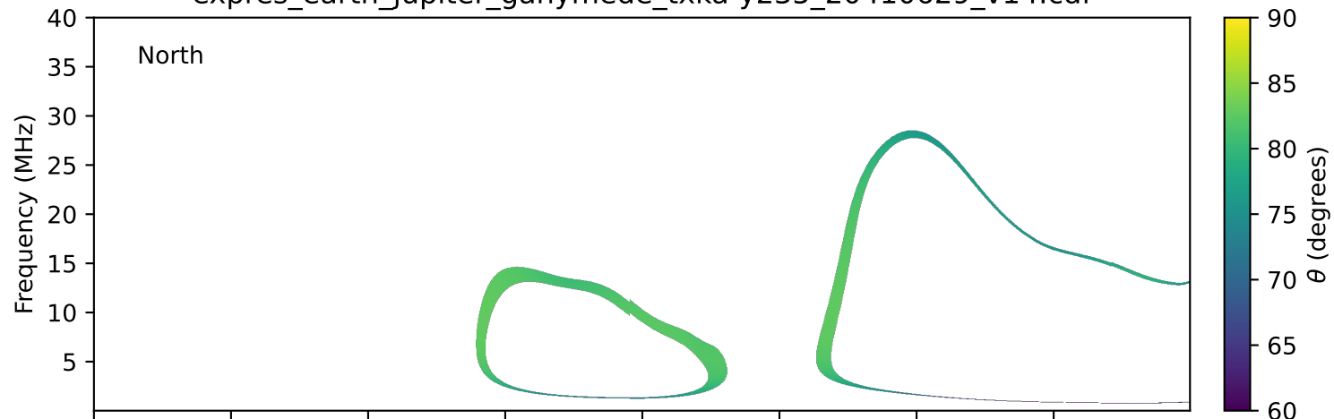
expres_earth_jupiter_ganymede_txka-y235_20410629_v14.cdf
