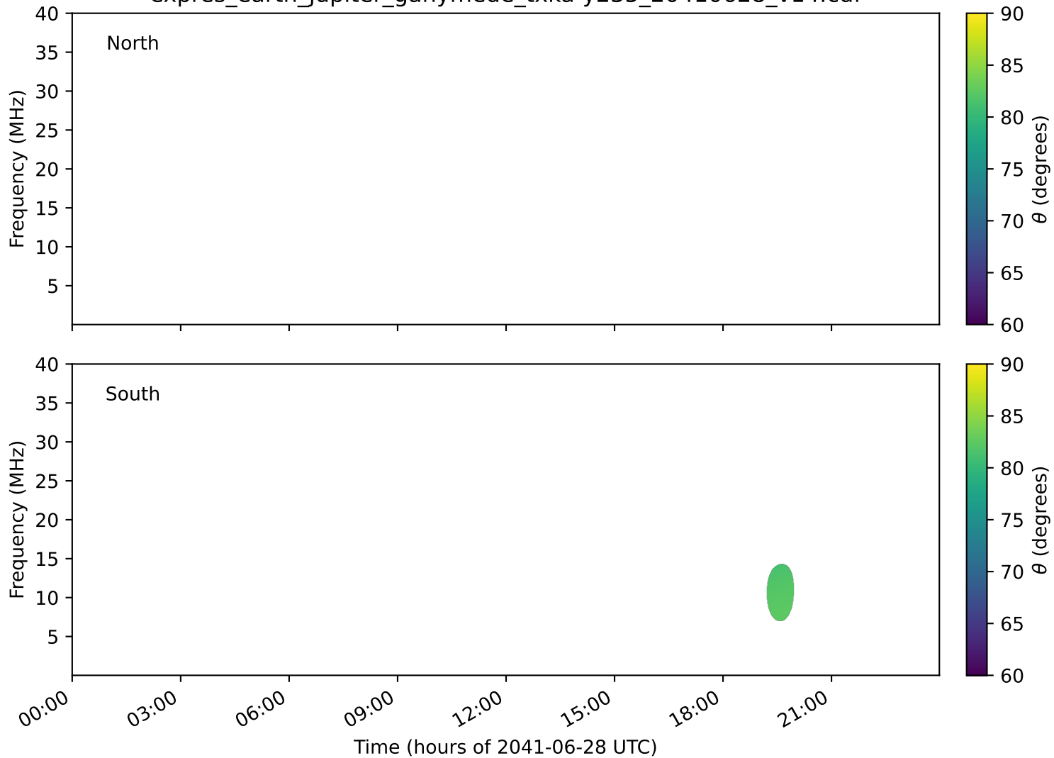
expres_earth_jupiter_ganymede_txka-y235_20410628_v14.cdf
