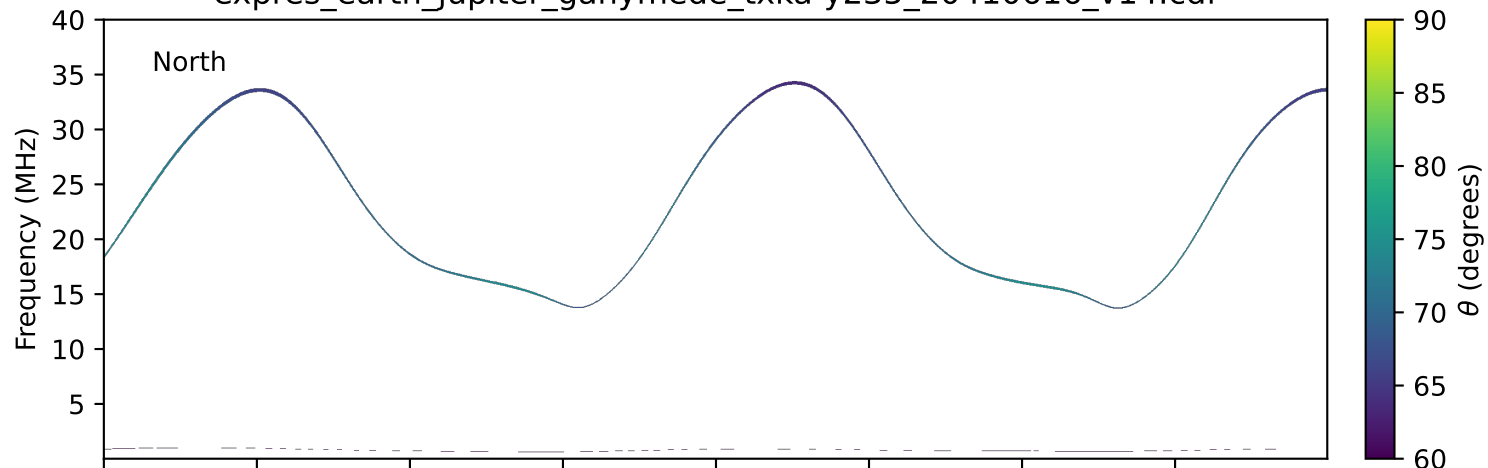
expres_earth_jupiter_ganymede_txka-y235_20410616_v14.cdf
