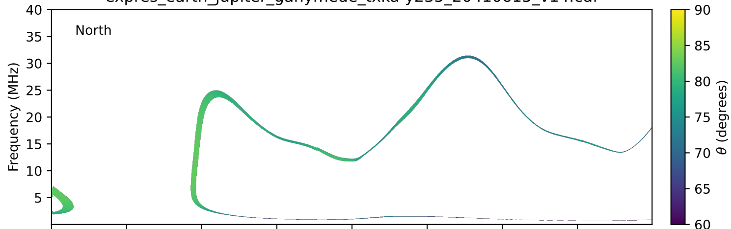
expres_earth_jupiter_ganymede_txka-y235_20410615_v14.cdf
