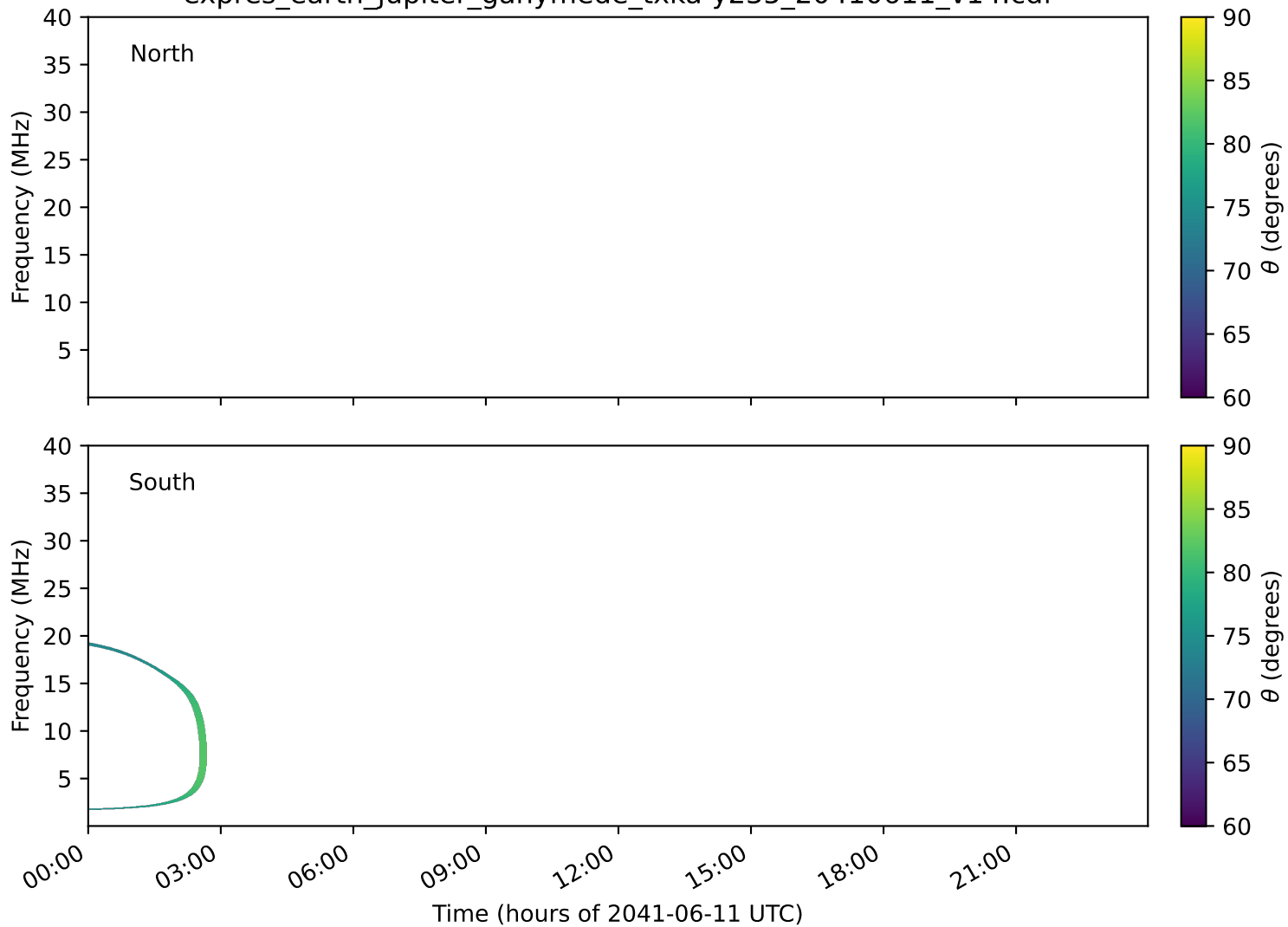
expres_earth_jupiter_ganymede_txka-y235_20410611_v14.cdf
