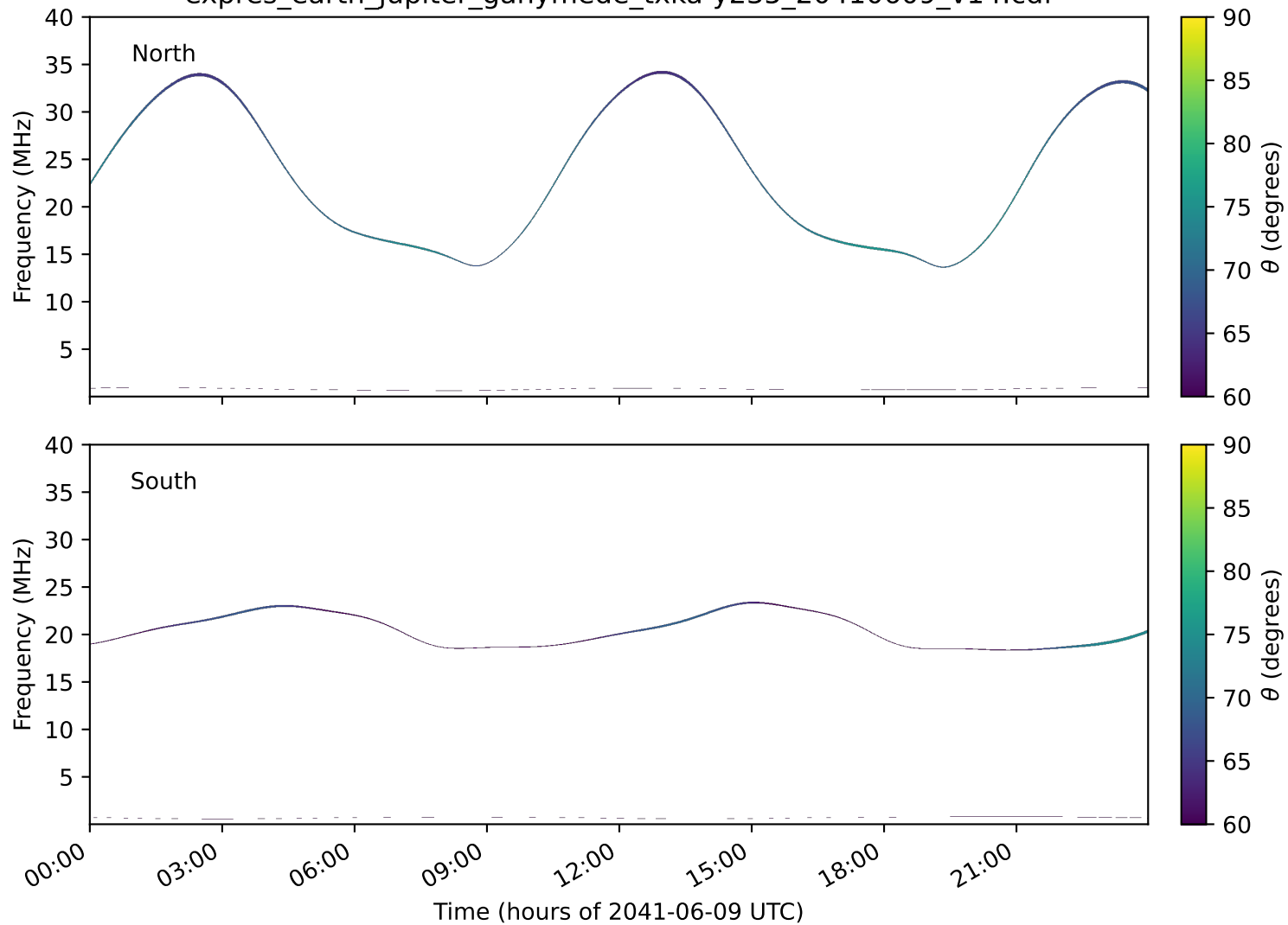
expres_earth_jupiter_ganymede_txka-y235_20410609_v14.cdf
