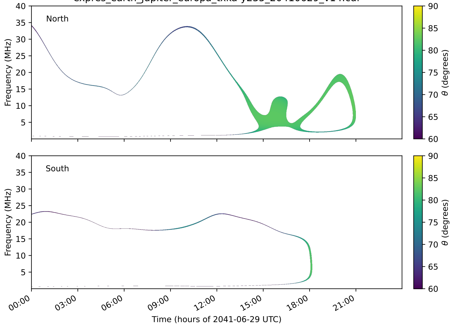
expres_earth_jupiter_europa_txka-y235_20410629_v14.cdf
