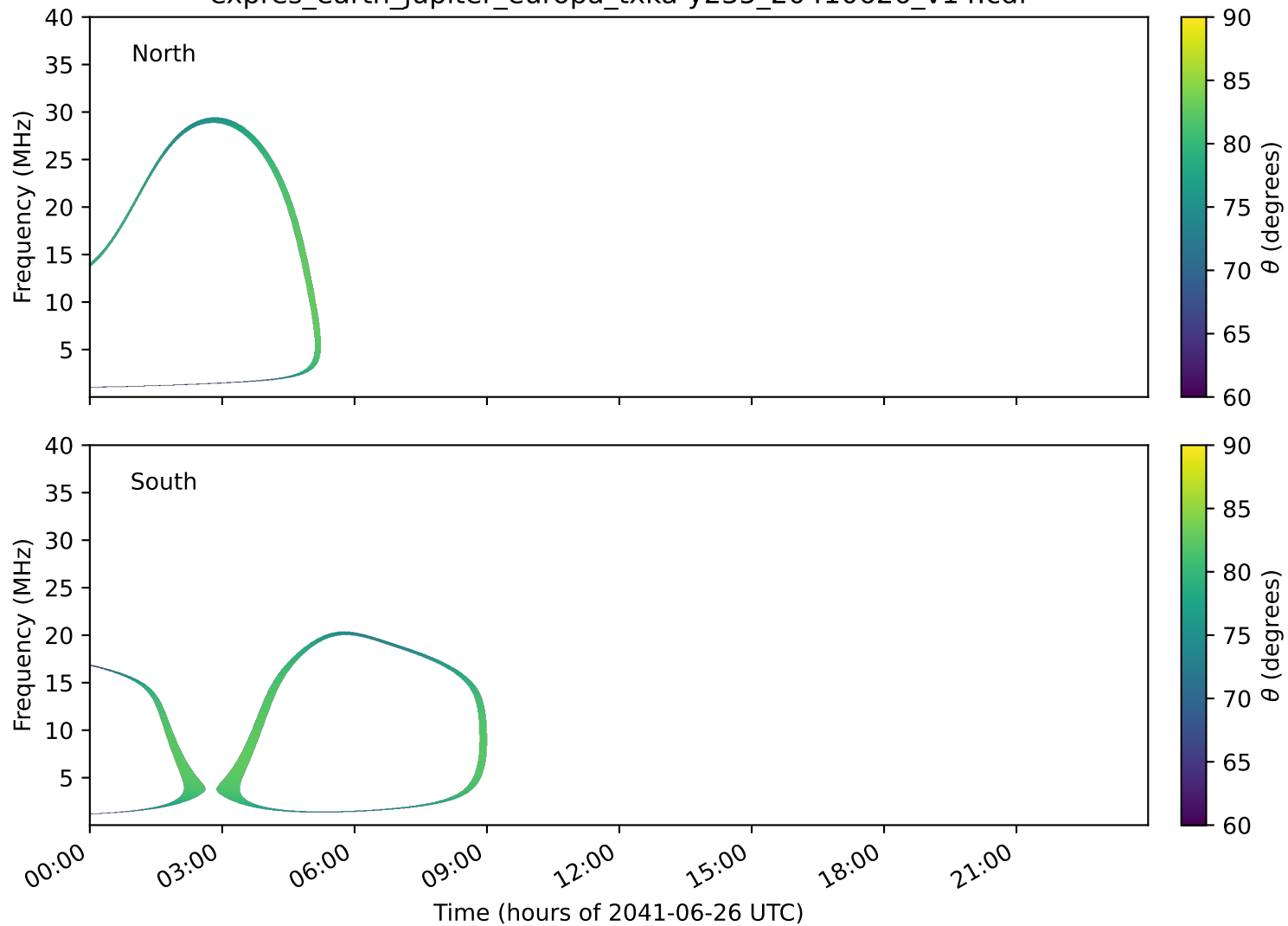
expres_earth_jupiter_europa_txka-y235_20410626_v14.cdf
