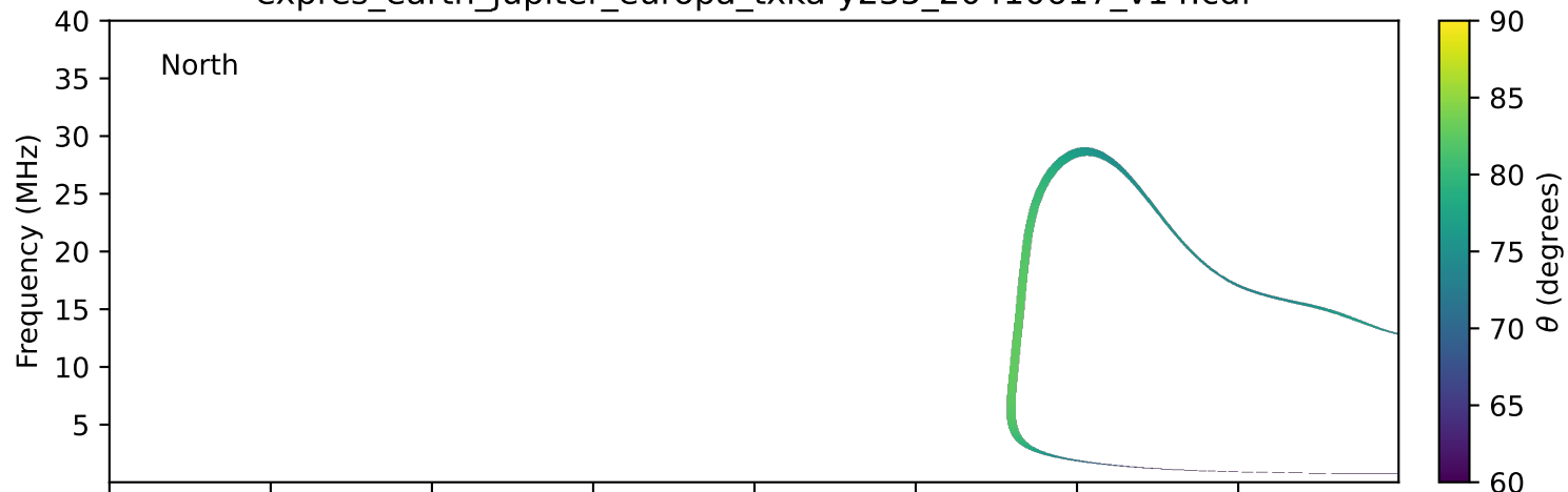
expres_earth_jupiter_europa_txka-y235_20410617_v14.cdf
