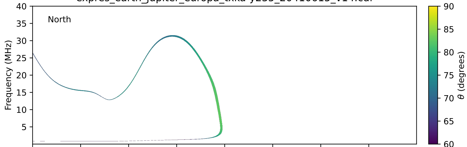
expres_earth_jupiter_europa_txka-y235_20410615_v14.cdf
