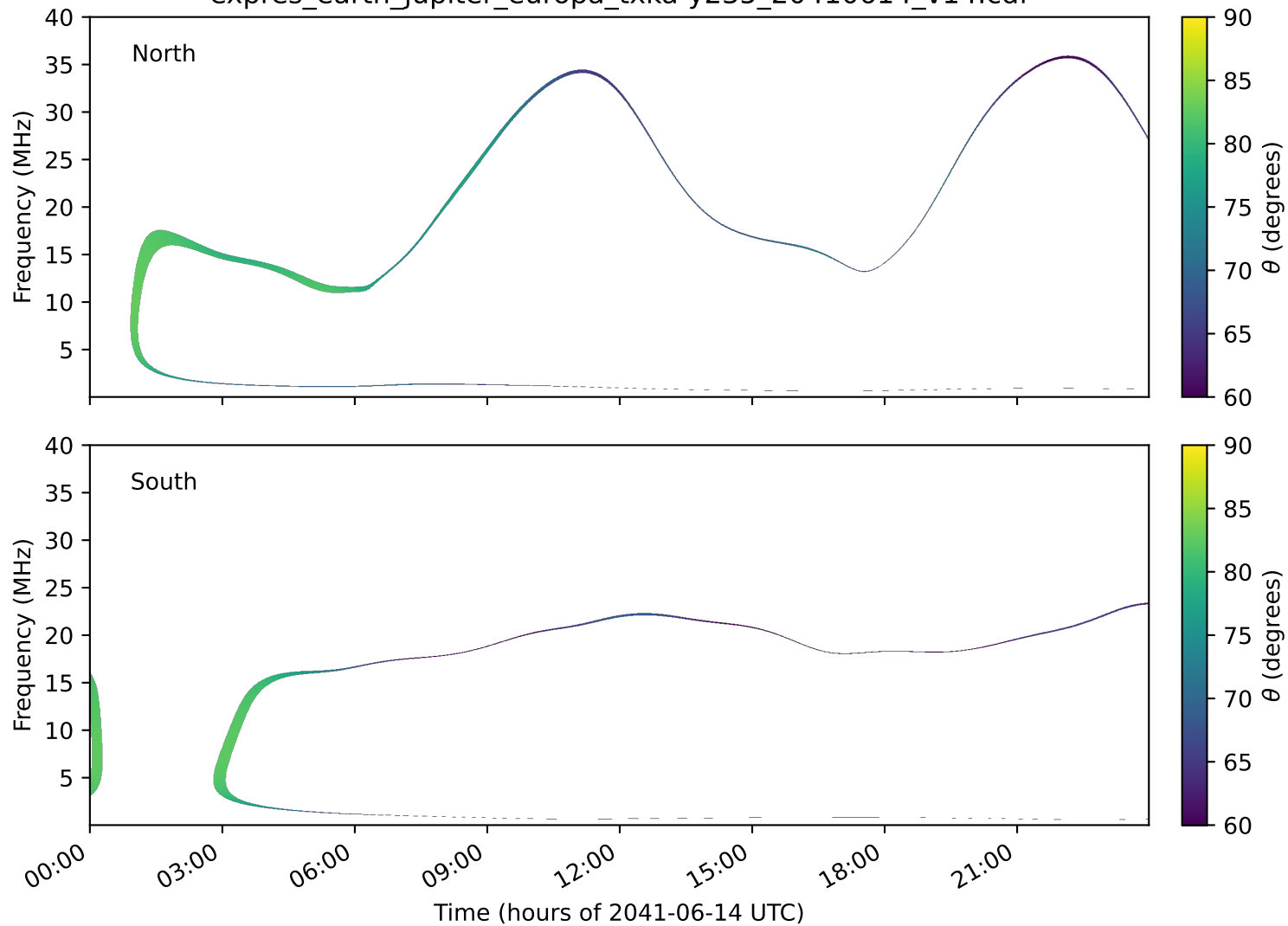
expres_earth_jupiter_europa_txka-y235_20410614_v14.cdf
