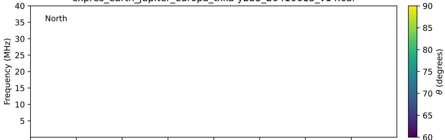
expres_earth_jupiter_europa_txka-y235_20410613_v14.cdf
