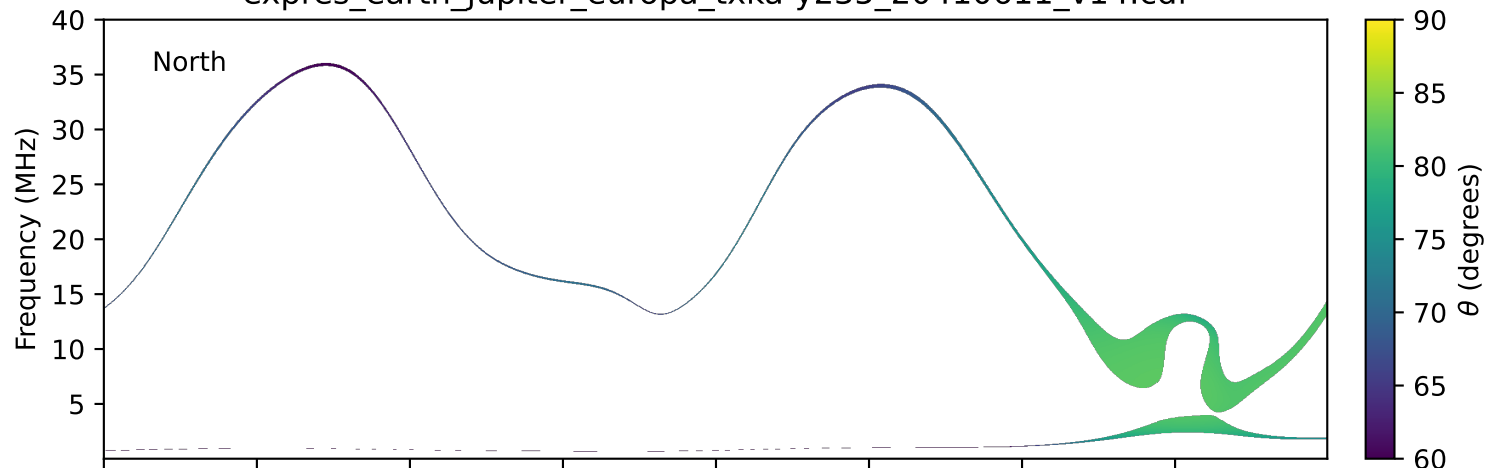
expres_earth_jupiter_europa_txka-y235_20410611_v14.cdf
