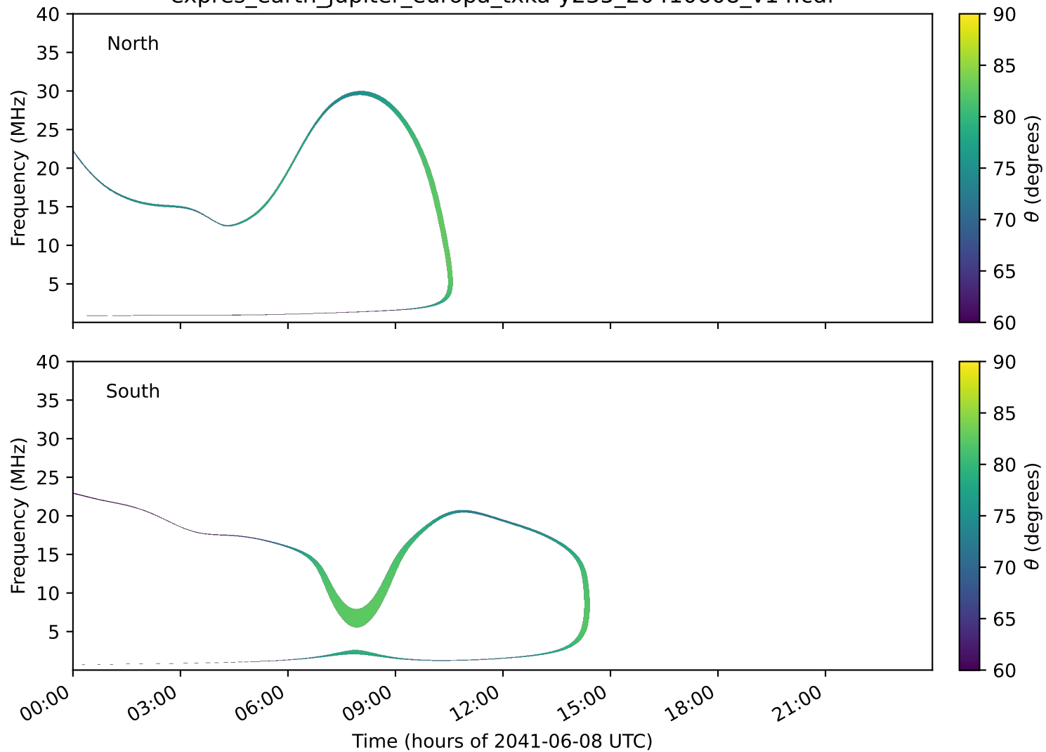
expres_earth_jupiter_europa_txka-y235_20410608_v14.cdf
