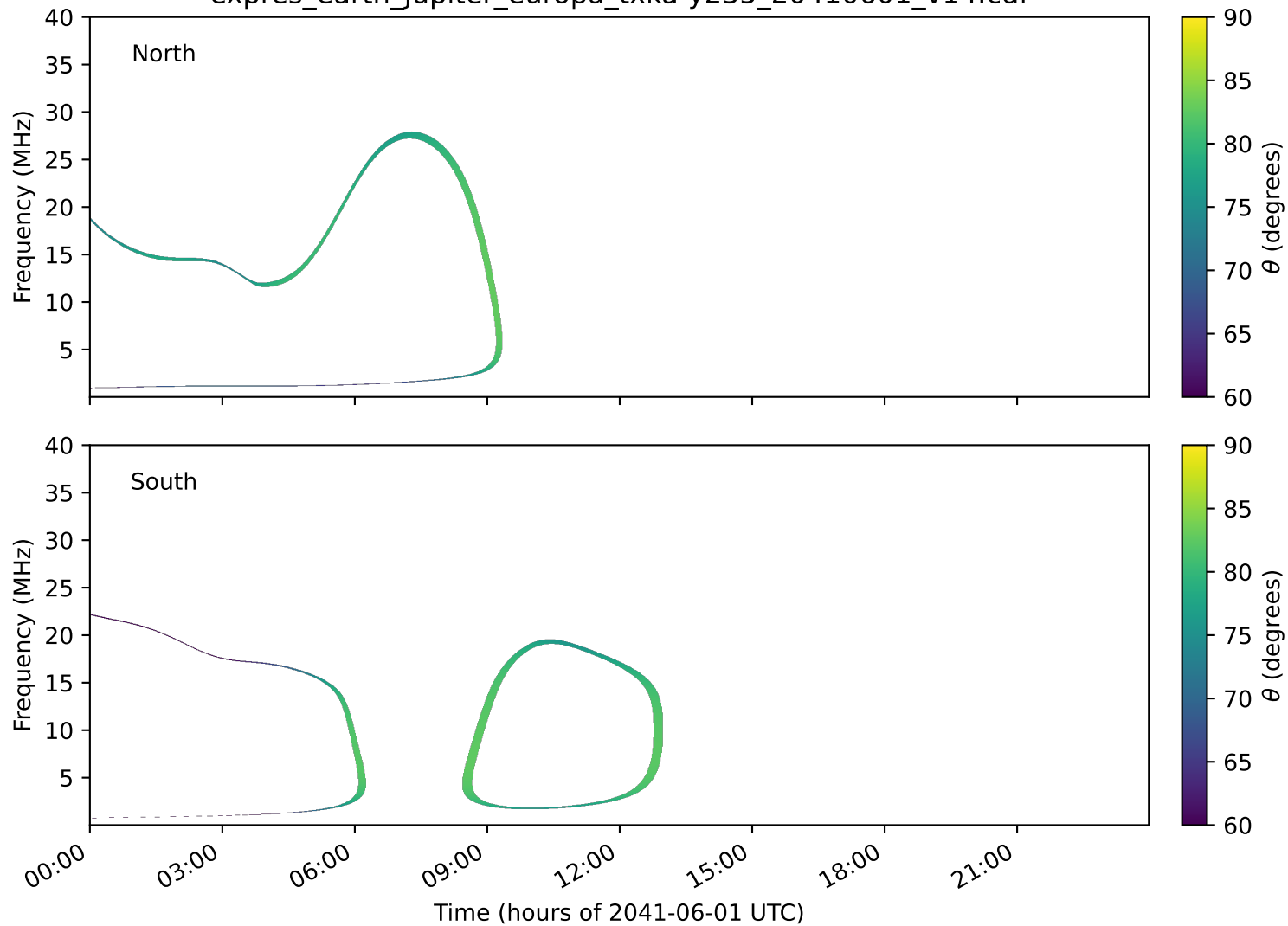
expres_earth_jupiter_europa_txka-y235_20410601_v14.cdf
