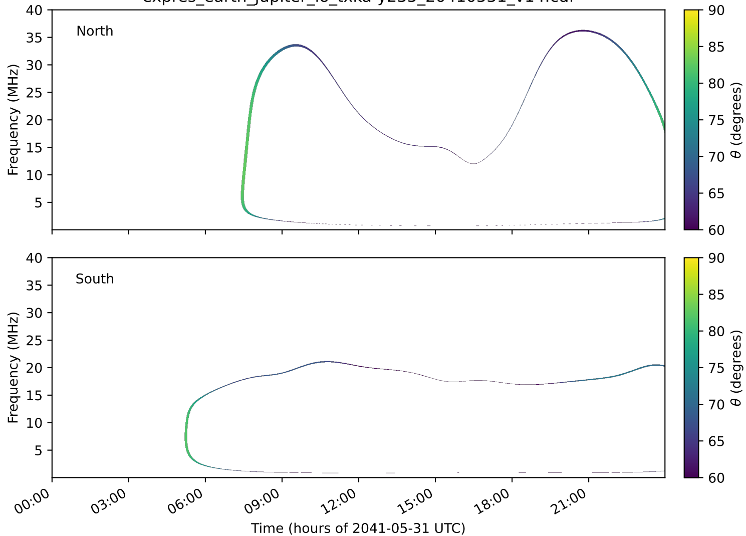
expres_earth_jupiter_io_txka-y235_20410531_v14.cdf
