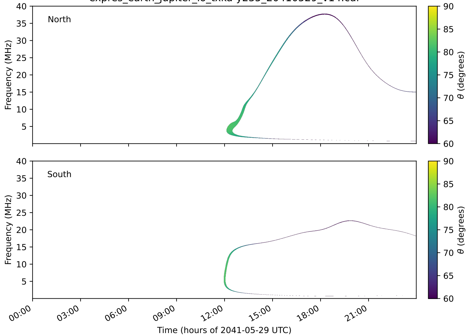
expres_earth_jupiter_io_txka-y235_20410529_v14.cdf
