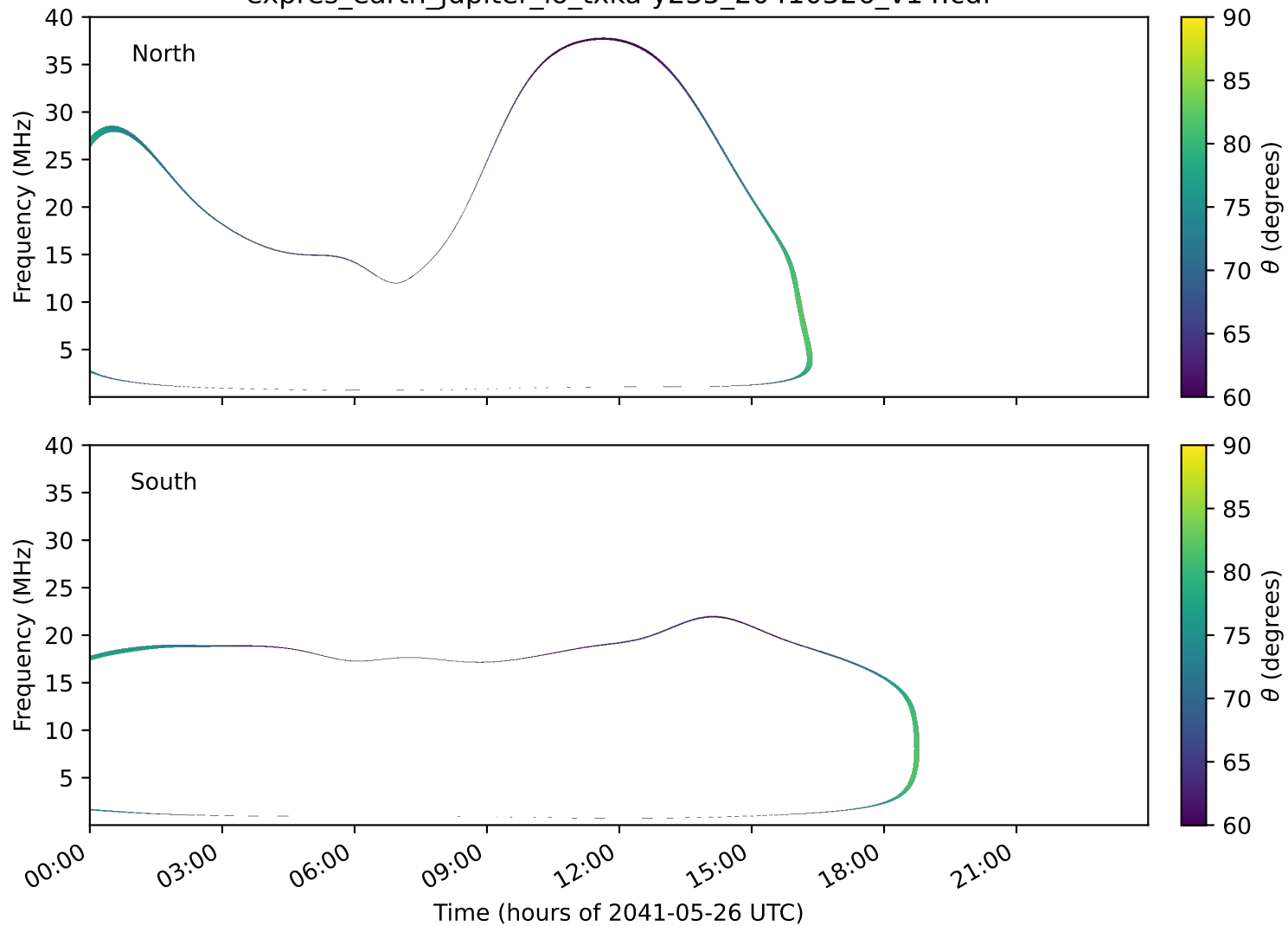
expres_earth_jupiter_io_txka-y235_20410526_v14.cdf
