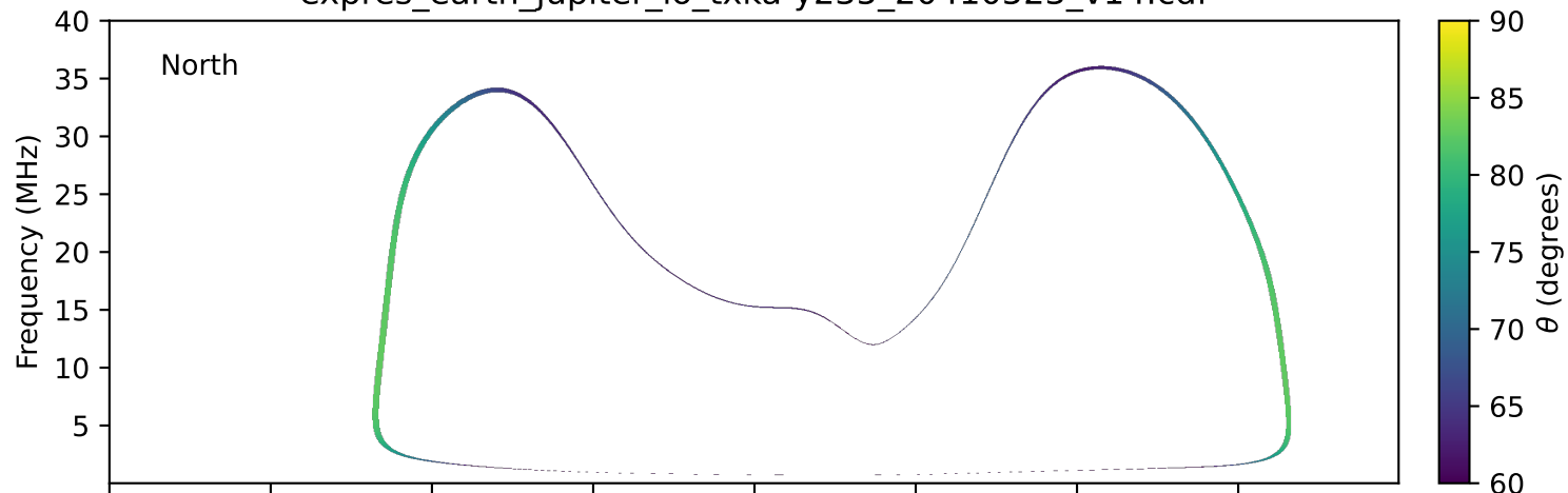
expres_earth_jupiter_io_txka-y235_20410523_v14.cdf
