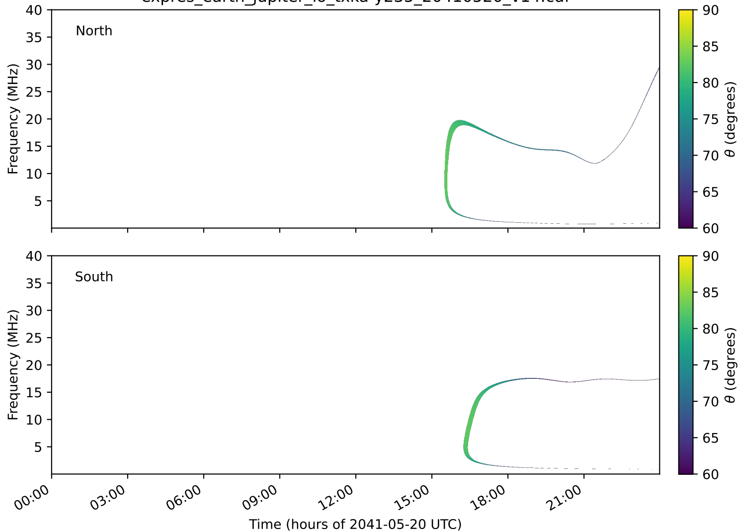
expres_earth_jupiter_io_txka-y235_20410520_v14.cdf
