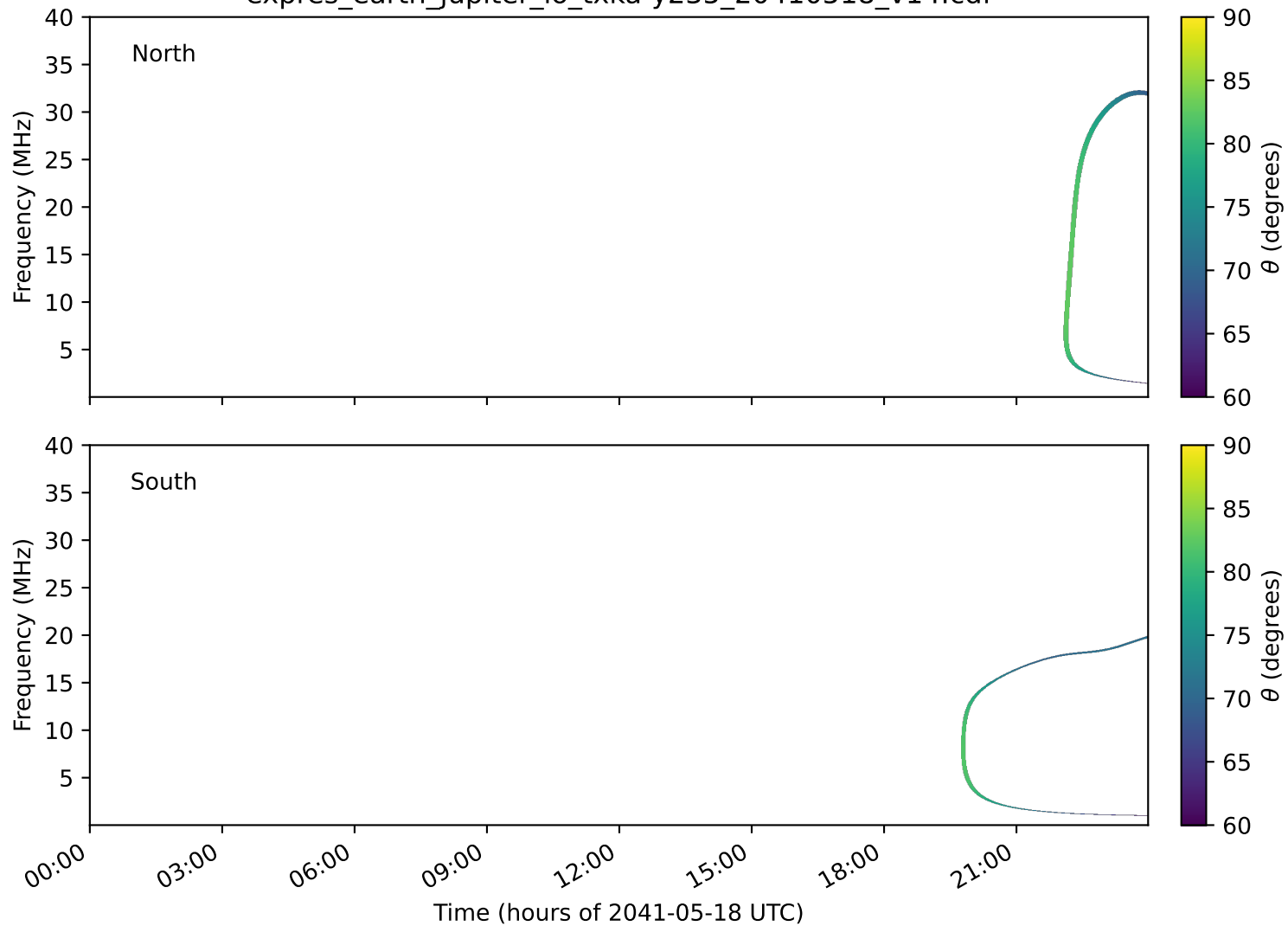
expres_earth_jupiter_io_txka-y235_20410518_v14.cdf
