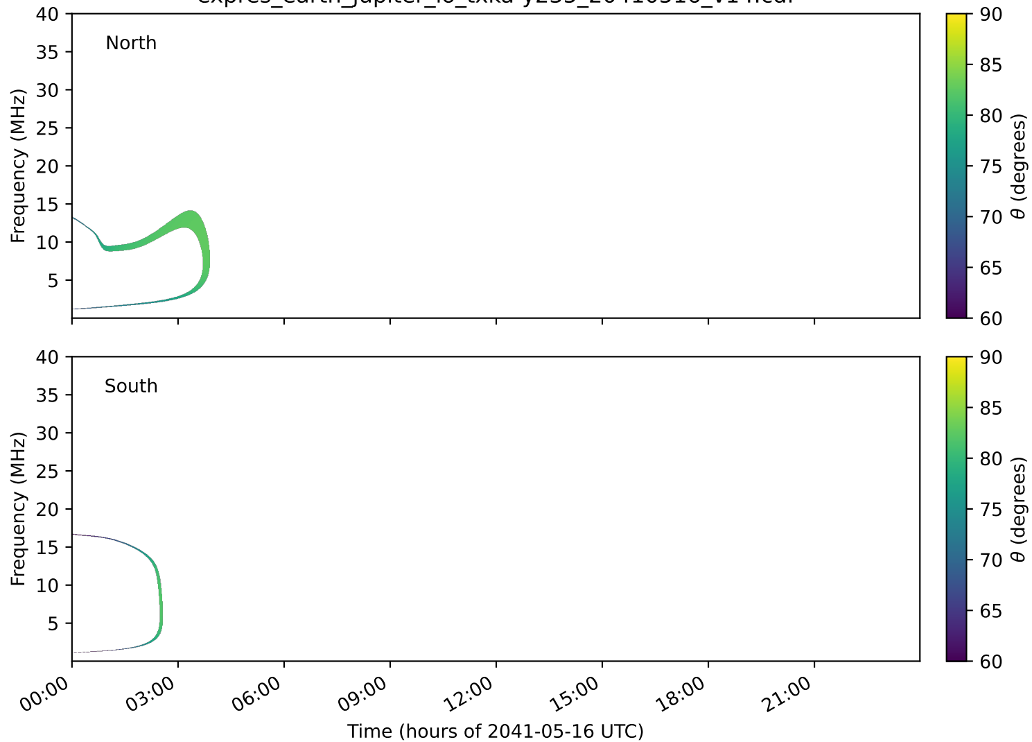
expres_earth_jupiter_io_txka-y235_20410516_v14.cdf
