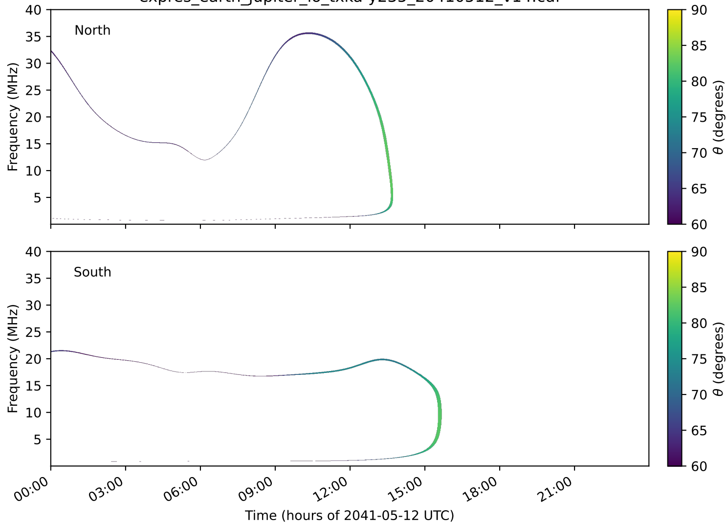
expres_earth_jupiter_io_txka-y235_20410512_v14.cdf
