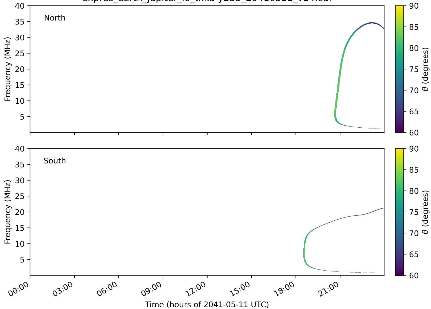
expres_earth_jupiter_io_txka-y235_20410511_v14.cdf
