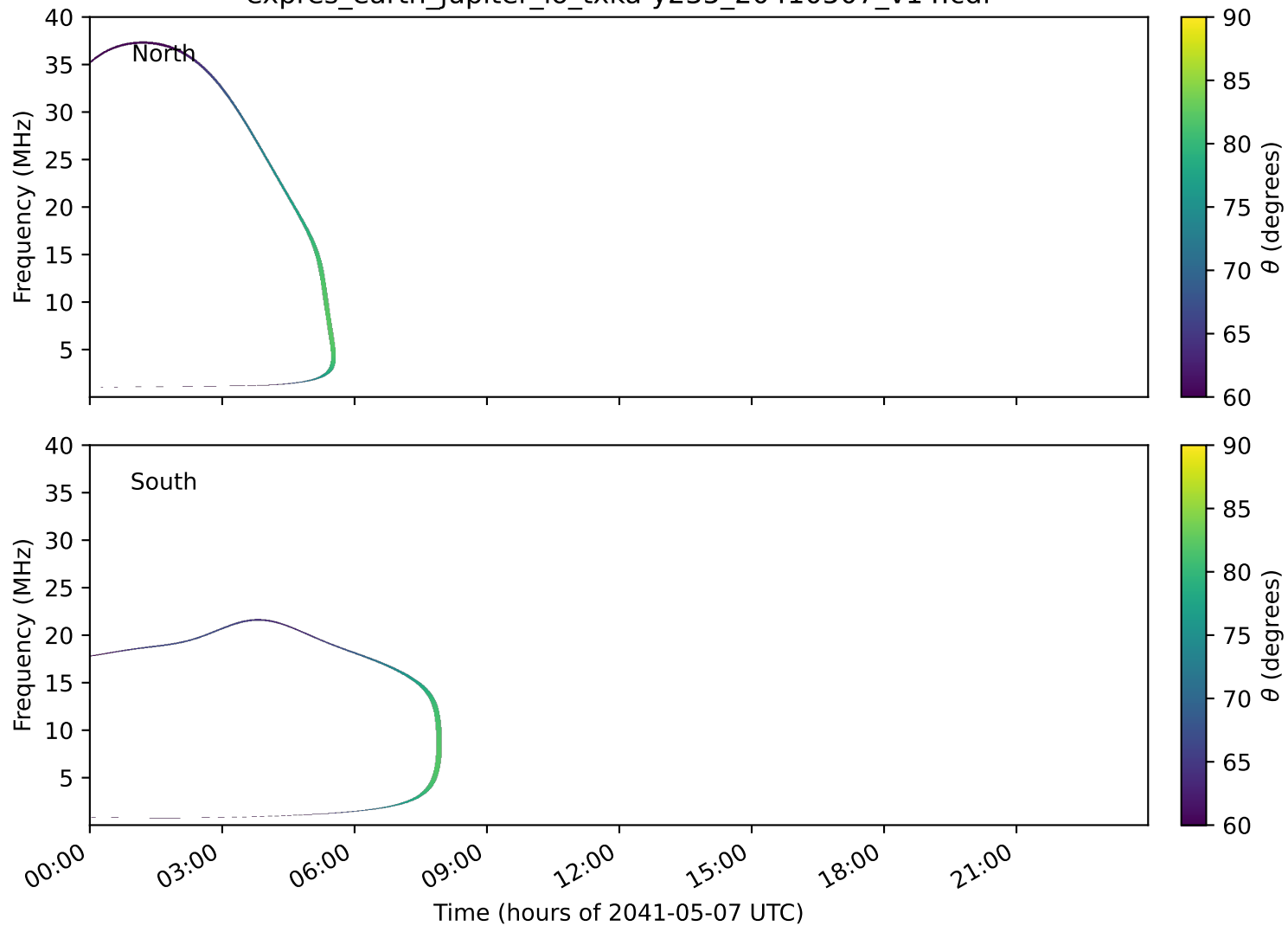
expres_earth_jupiter_io_txka-y235_20410507_v14.cdf
