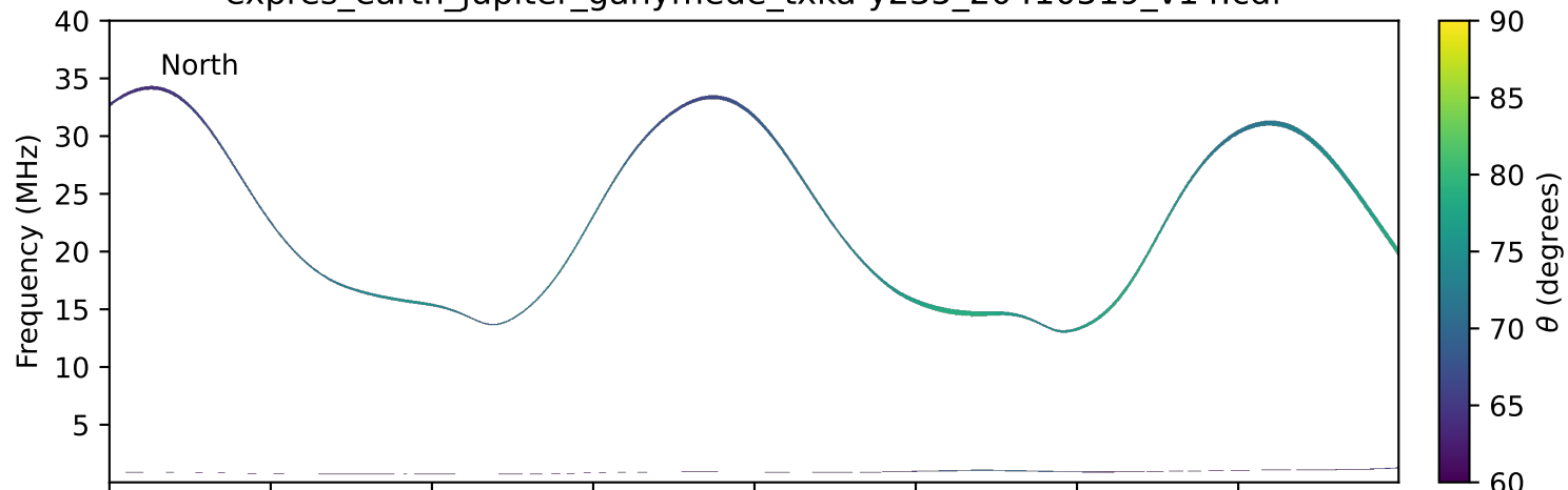
expres_earth_jupiter_ganymede_txka-y235_20410519_v14.cdf
