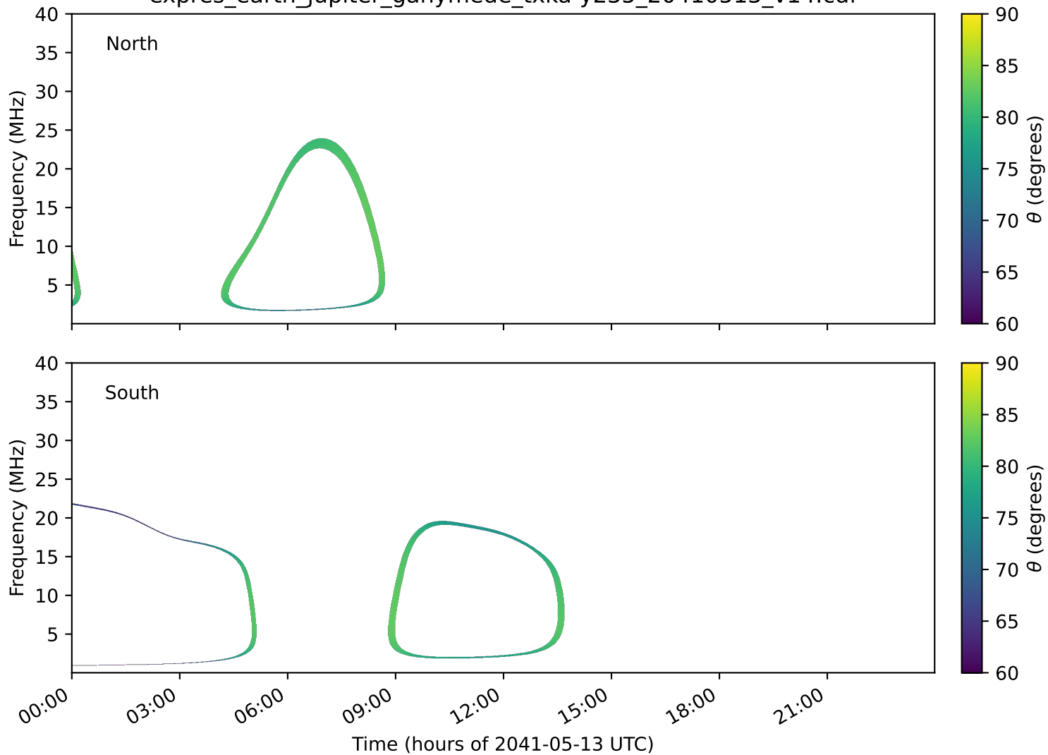
expres_earth_jupiter_ganymede_txka-y235_20410513_v14.cdf
