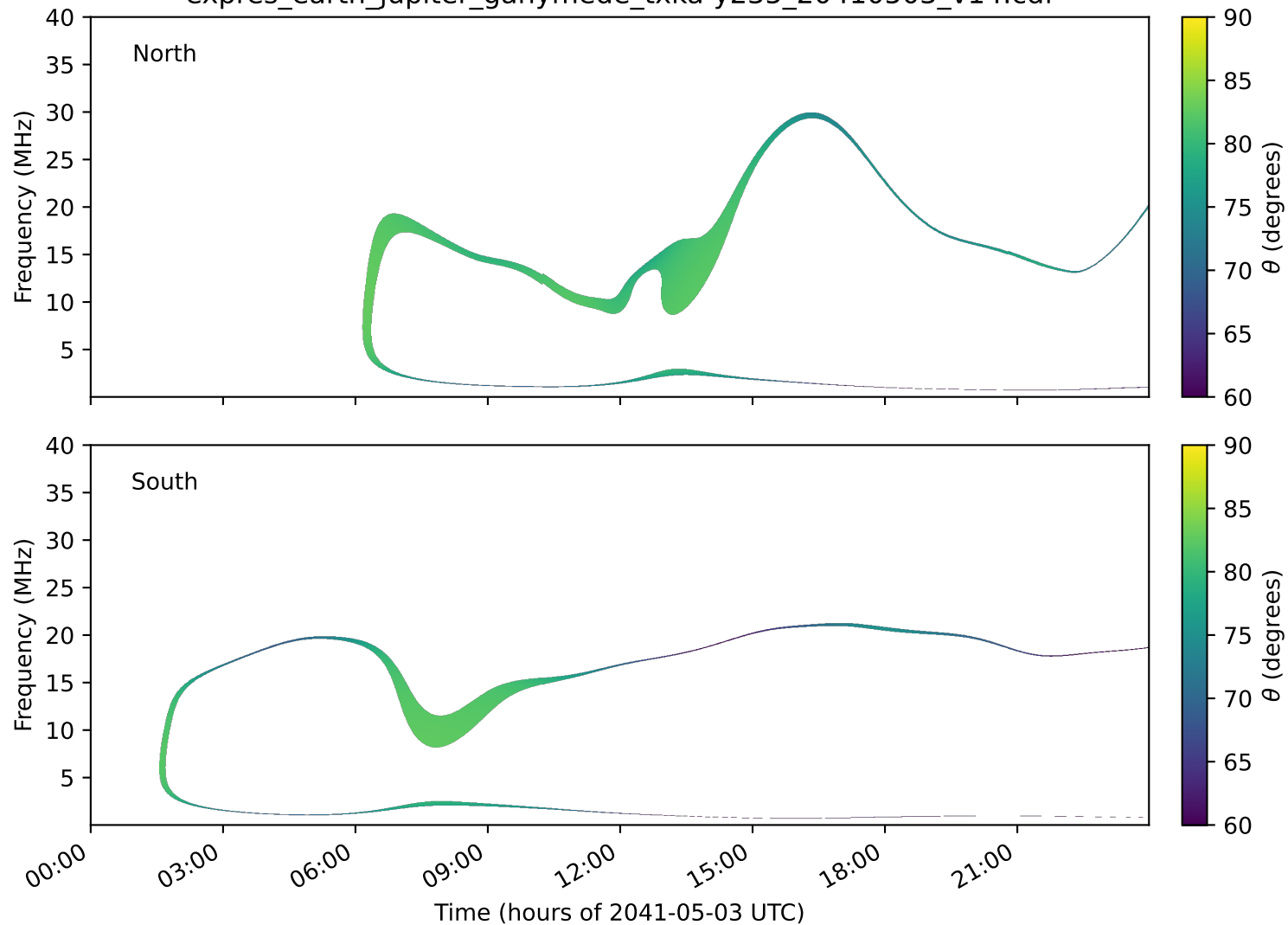
expres_earth_jupiter_ganymede_txka-y235_20410503_v14.cdf
