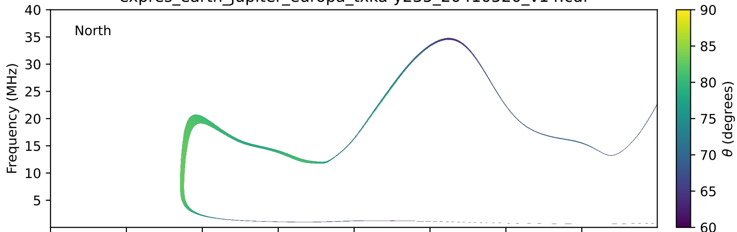
expres_earth_jupiter_europa_txka-y235_20410520_v14.cdf
