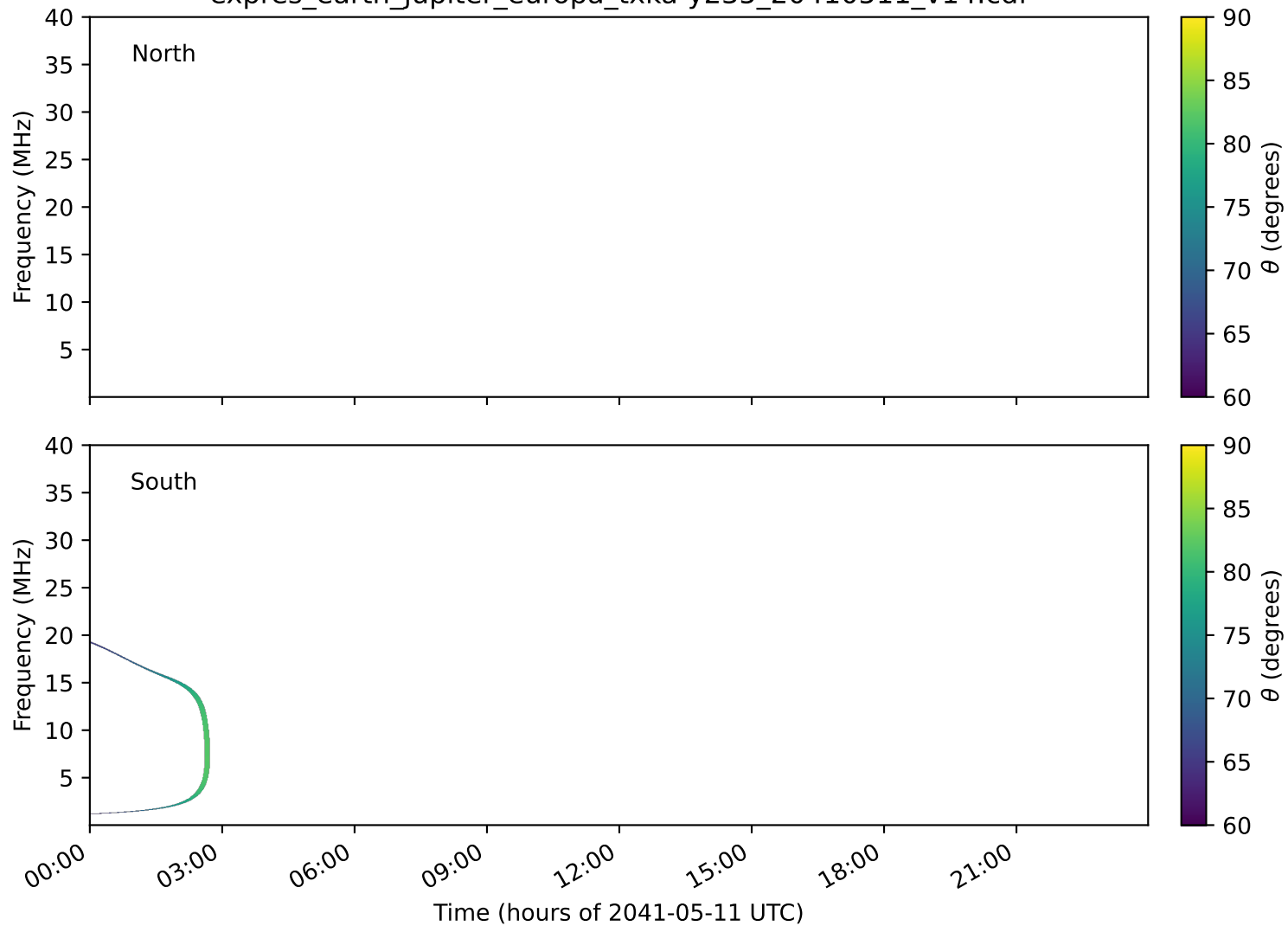
expres_earth_jupiter_europa_txka-y235_20410511_v14.cdf
