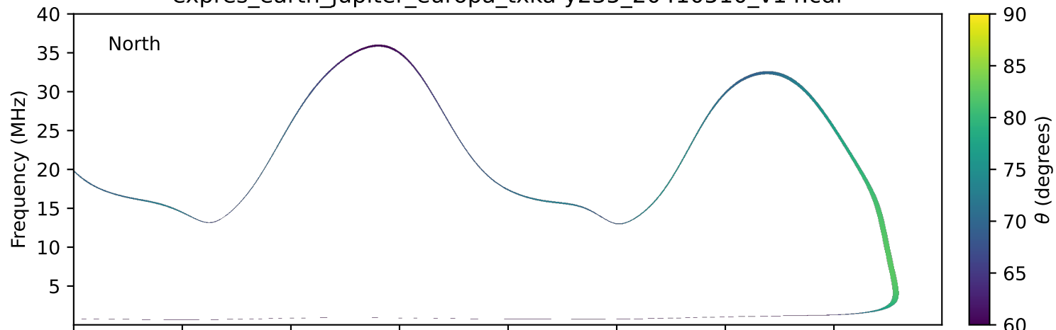
expres_earth_jupiter_europa_txka-y235_20410510_v14.cdf
