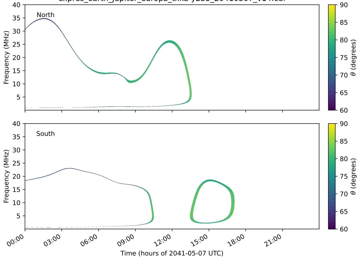
expres_earth_jupiter_europa_txka-y235_20410507_v14.cdf
