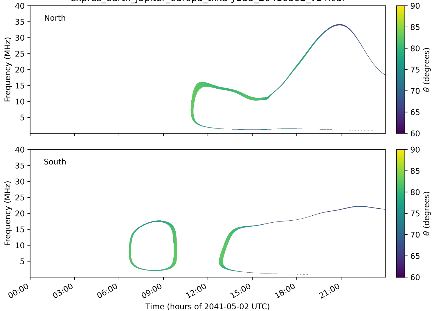
expres_earth_jupiter_europa_txka-y235_20410502_v14.cdf
