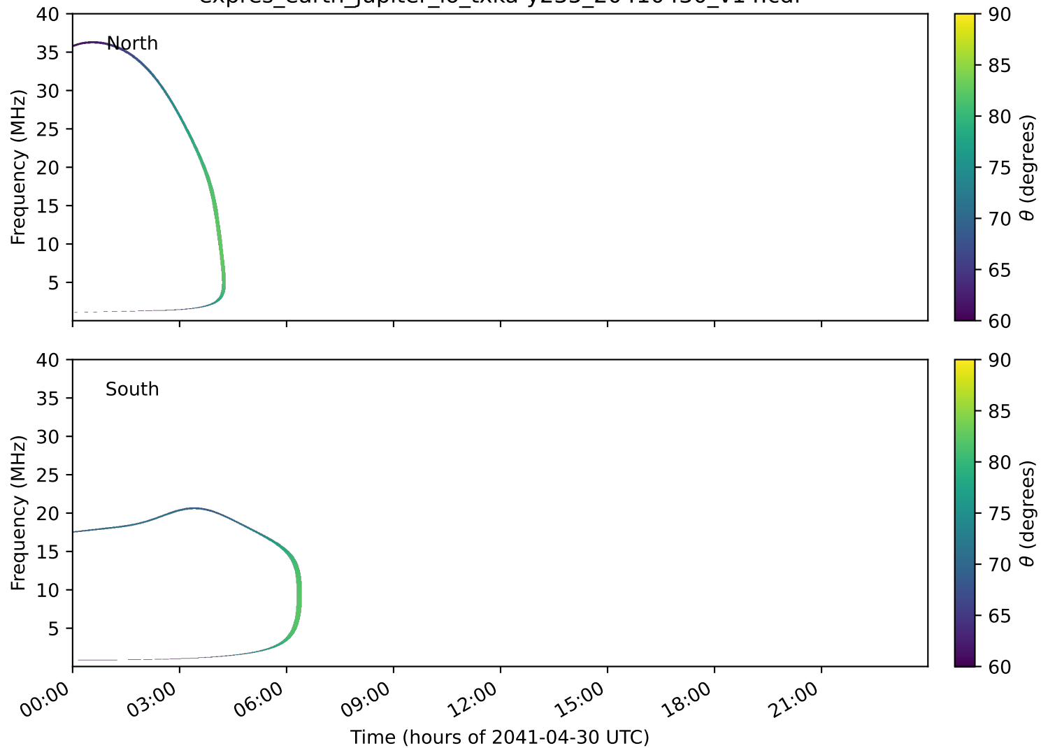
expres_earth_jupiter_io_txka-y235_20410430_v14.cdf
