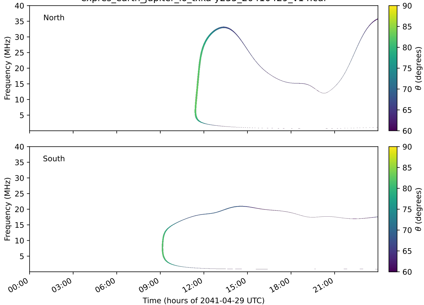
expres_earth_jupiter_io_txka-y235_20410429_v14.cdf
