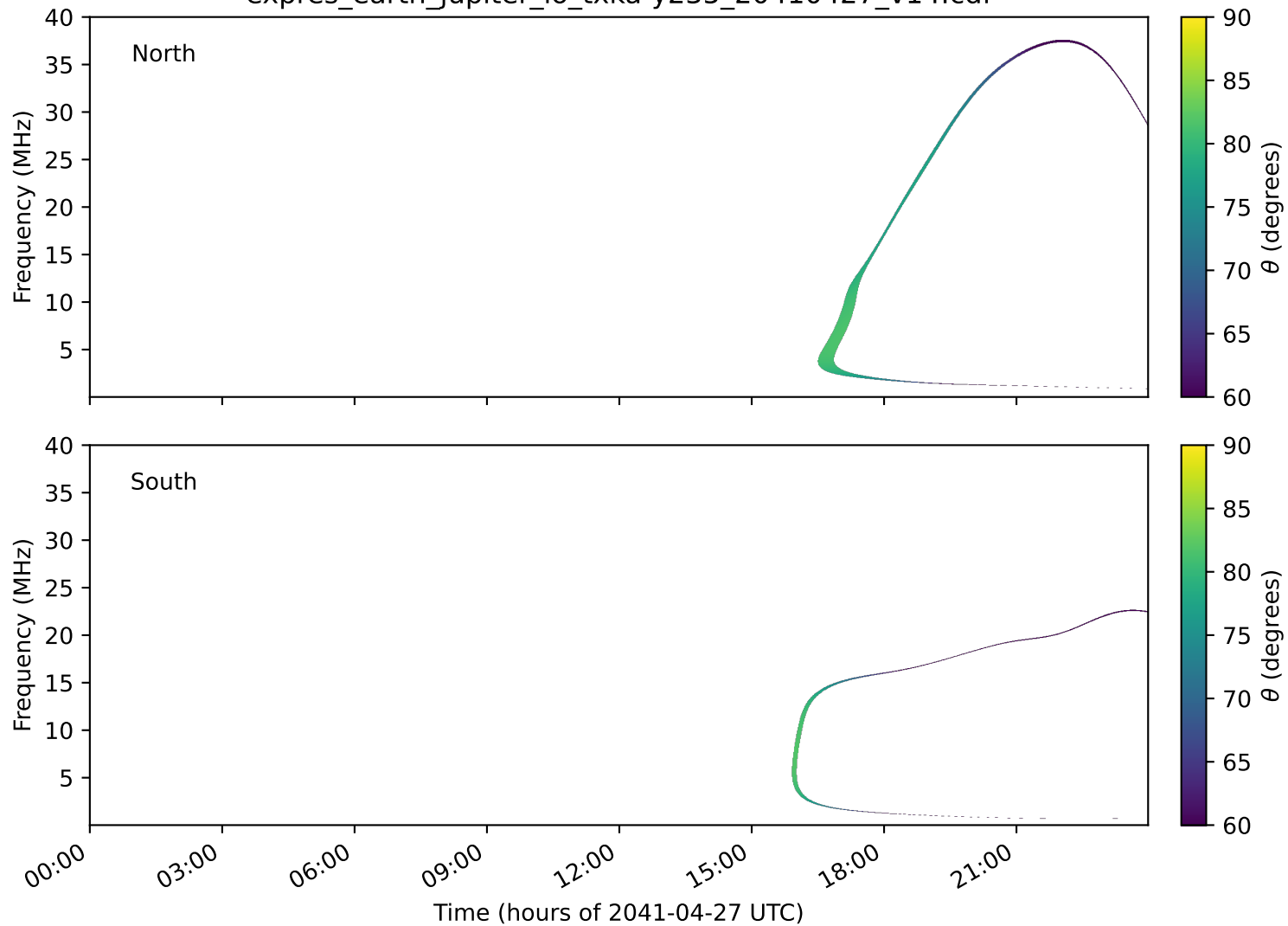
expres_earth_jupiter_io_txka-y235_20410427_v14.cdf
