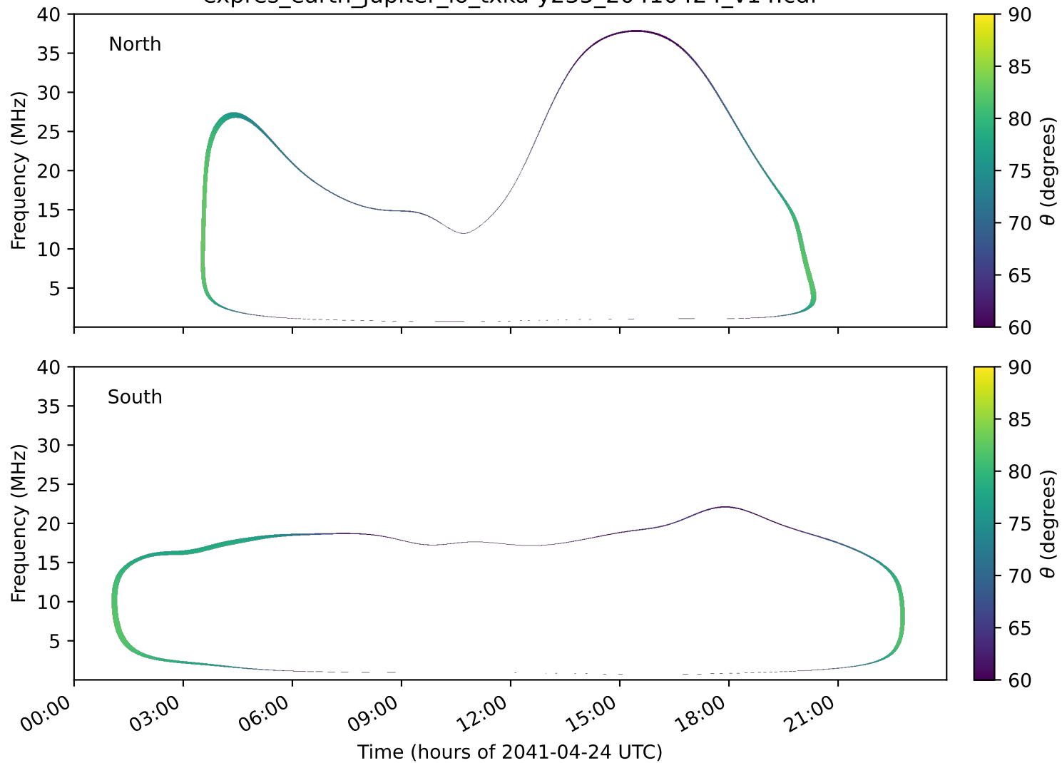
expres_earth_jupiter_io_txka-y235_20410424_v14.cdf
