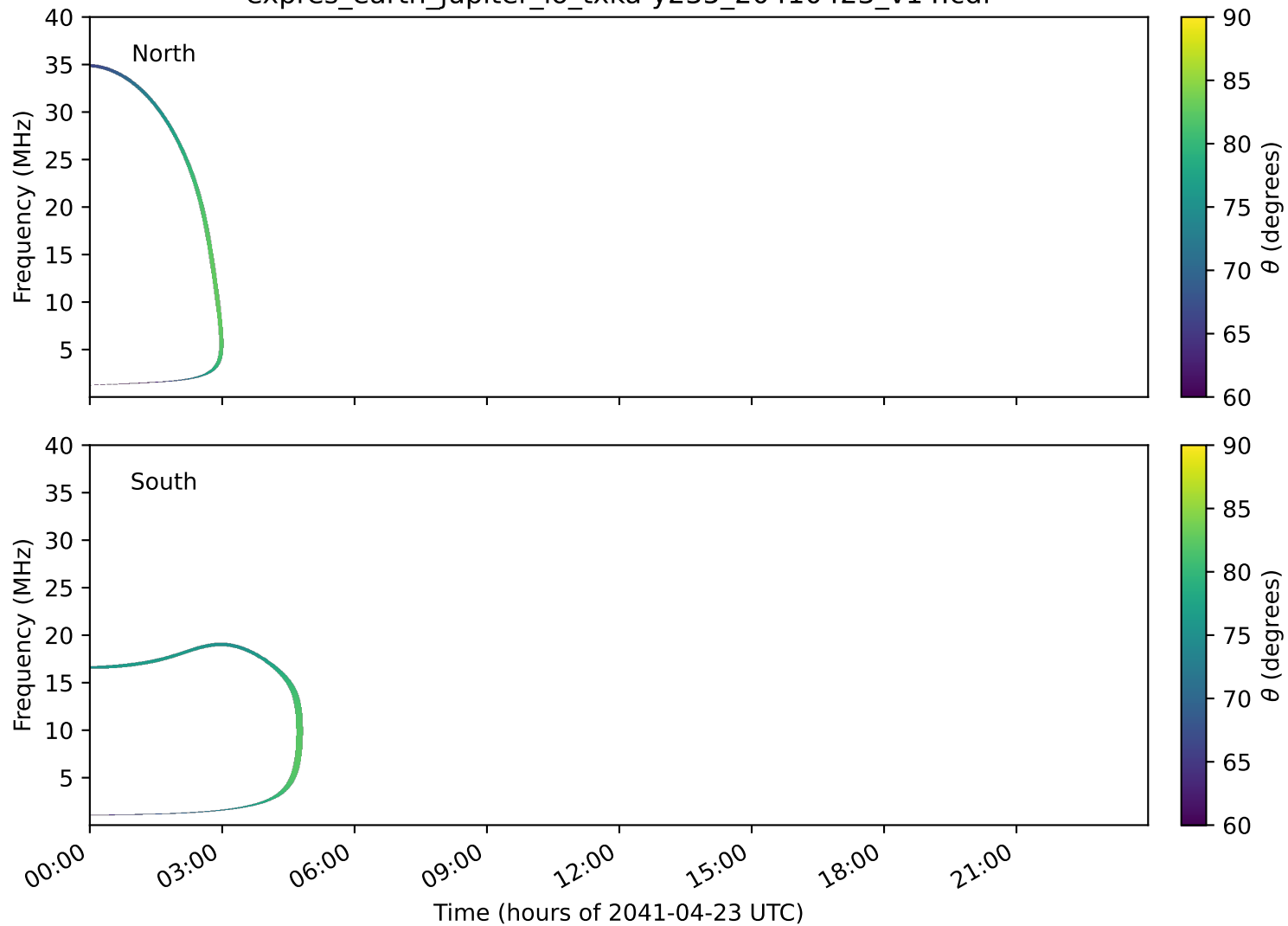
expres_earth_jupiter_io_txka-y235_20410423_v14.cdf
