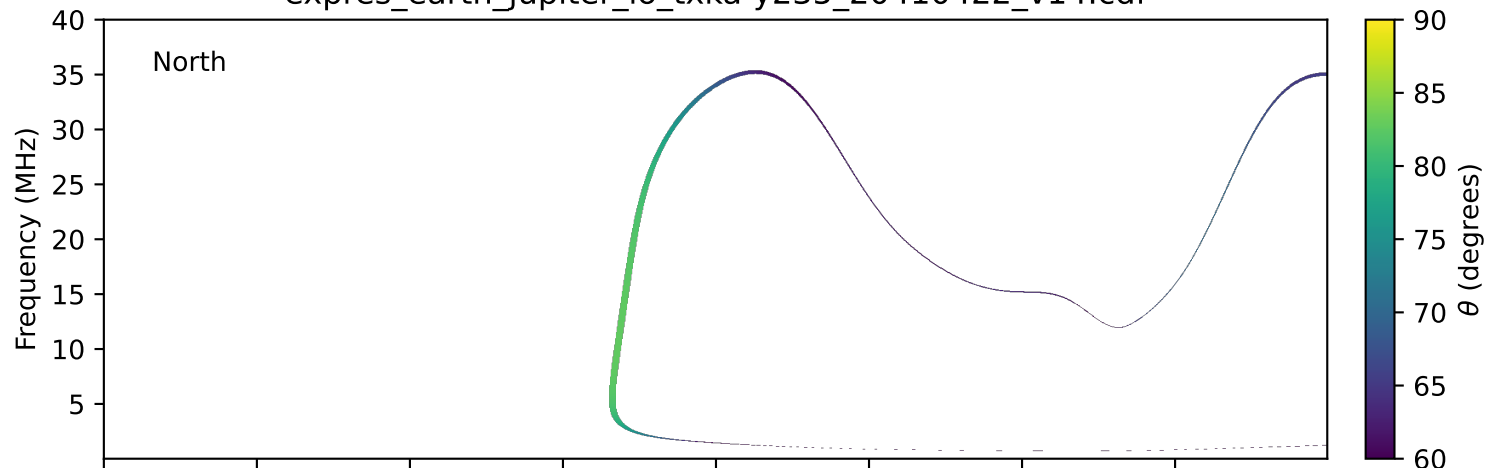
expres_earth_jupiter_io_txka-y235_20410422_v14.cdf
