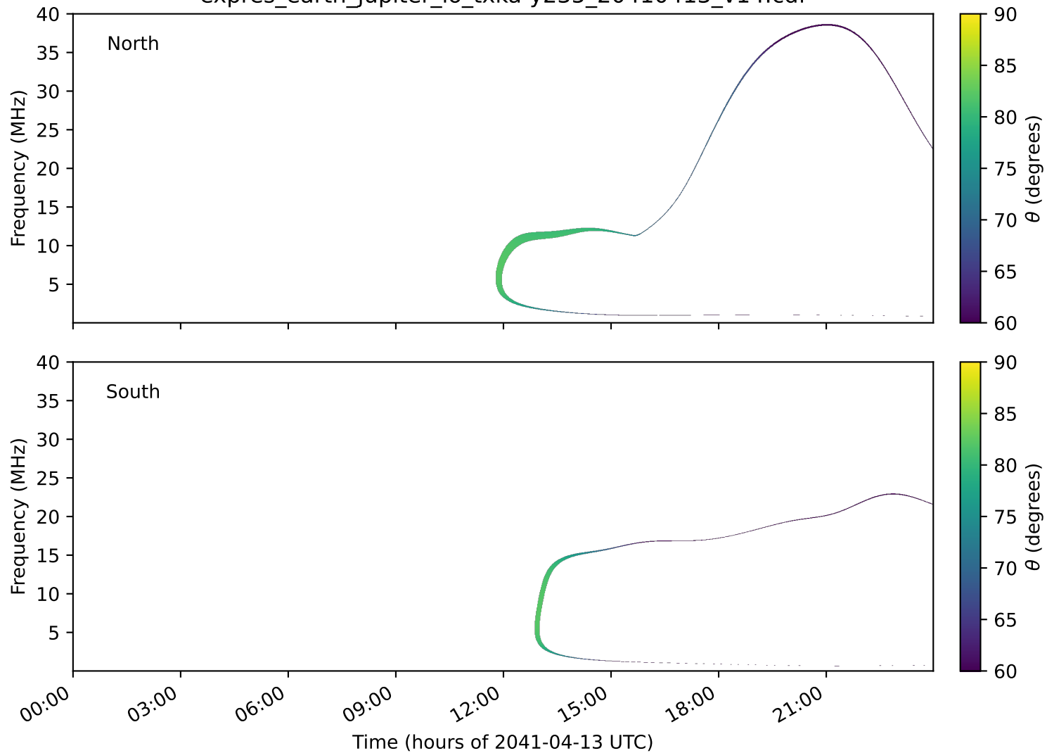
expres_earth_jupiter_io_txka-y235_20410413_v14.cdf
