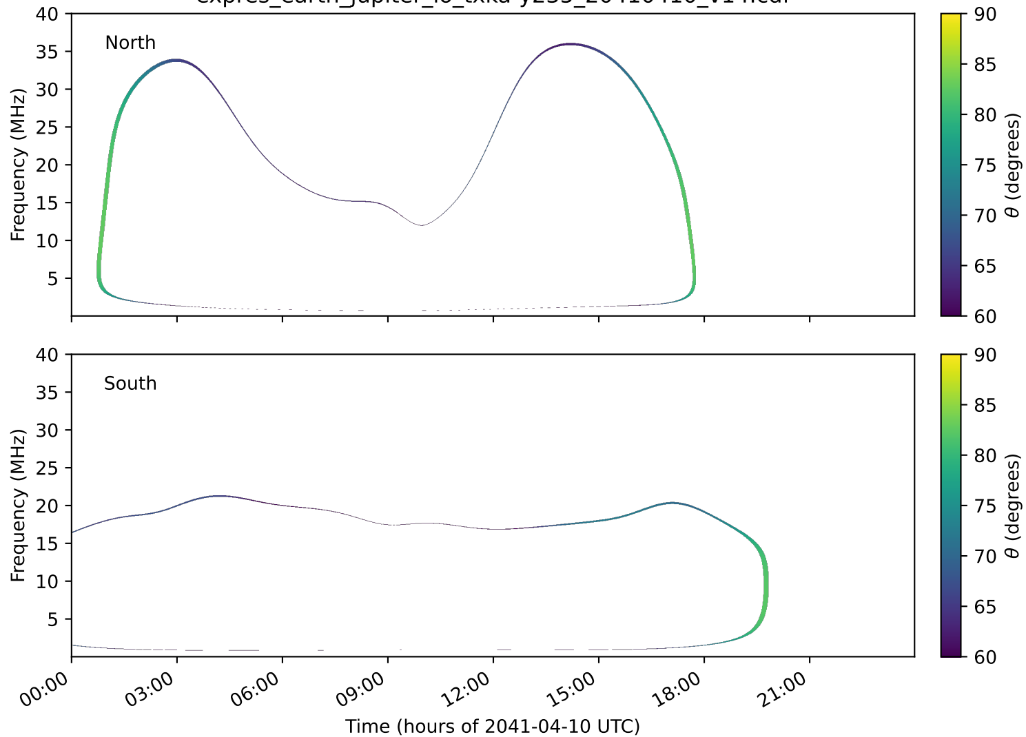
expres_earth_jupiter_io_txka-y235_20410410_v14.cdf
