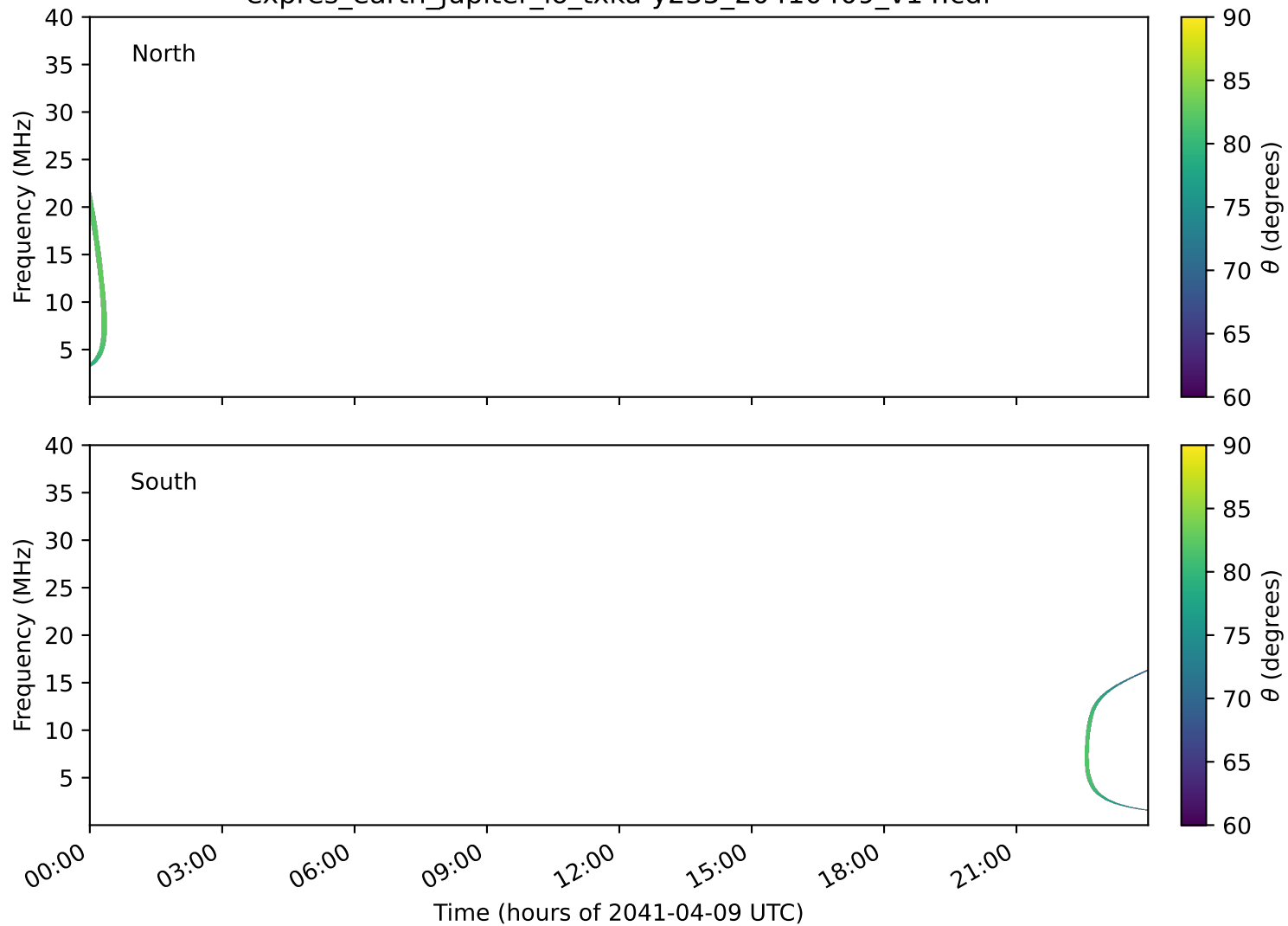
expres_earth_jupiter_io_txka-y235_20410409_v14.cdf
